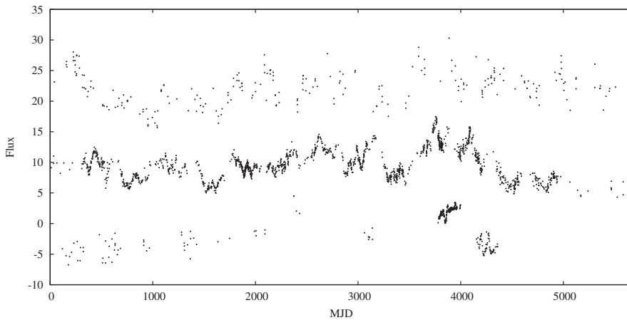
Figure 1. Folded phased diagram of NGC 5548 continuum flux 43 yr long light curve, assuming 5676 days periodicity, here presented to show an example of repeating noisy pattern light curve. Top light curve is pre AGN watch epoch, middle is AGN watch epoch Sergeev et al. (2007), and bottom is post AGN watch epoch constructed from new observations presented in Bon et al. (2016), Lu et al. (2016), Pei et al. (2017).
