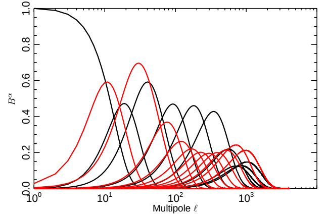
Fig. 1: Window functions corresponding to the spectral localisation of the NILC and MILCA algorithms. For NILC (black) there are 10 Gaussian window functions defining 10 needlet scales. MILCA (red) uses 11 Gaussian overlapping windows.
