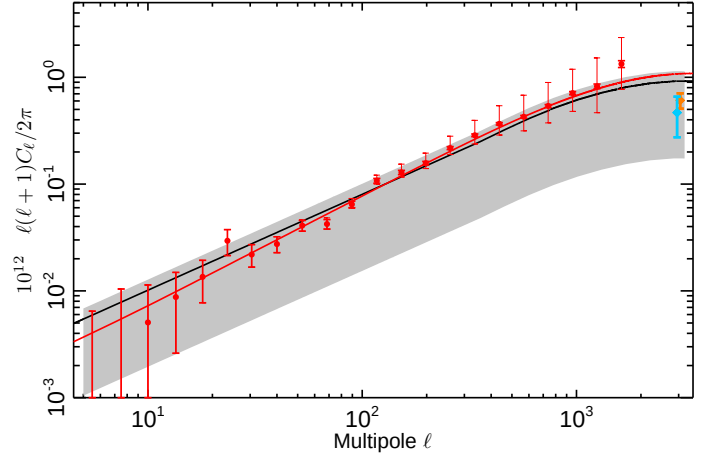
Fig. 17: NILC - MILCA F/L cross-power spectrum after foreground subtraction (red points), compared to the Atacama Cosmology Telescope (ACT; cyan dot) and the South Pole Telescope (SPT; orange, George et al., 2014) power spectrum estimates. The black line shows the tSZ power spectrum template (EM12 Efstathiou & Migliaccio, 2012) used in the Planck CMB cosmological analysis (Planck Collaboration XVI, 2014; Planck Collaboration XI, 2015) with its best fit amplitude A_{\text{tSZ}} (Planck Collaboration XI, 2015), the grey region allows comparison with the 2\sigma interval.
