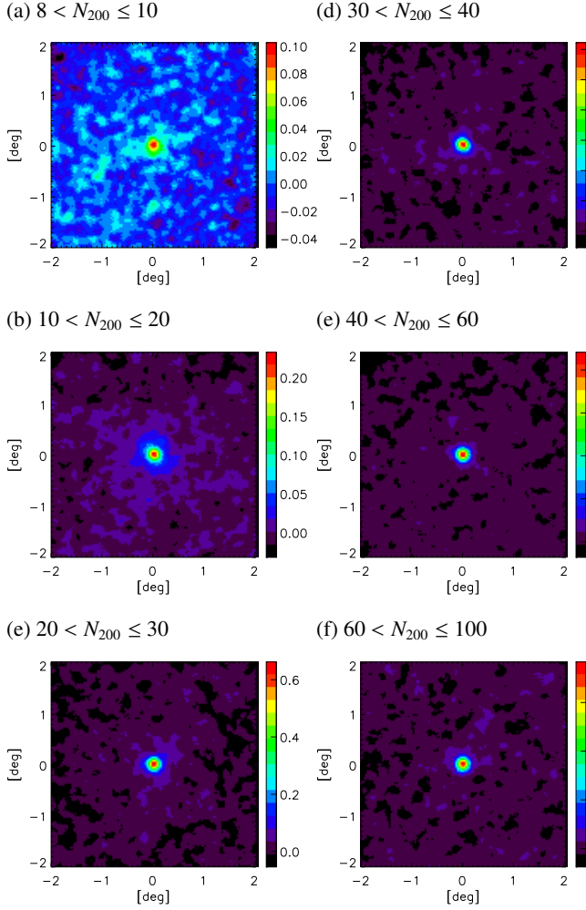
Fig. 9: 4^\circ \times 4^\circ average maps for different ranges in N_{200} from 8 to 100. The color scale is in unit of 10^{-6} y .
