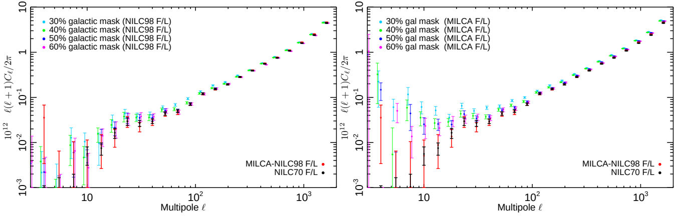
Fig. 11: Angular cross-power spectra of the Planck NILC F/L (left) and MILCA F/L (right) reconstructed Compton parameter maps for different Galactic masks corresponding to 30 % (cyan), 40 % (green), 50 % (blue) and 60 % (pink) of the sky. For comparison we also show MILCA-NILC F/L (red) and NILC70 F/L (black) on 50 % of the sky. See text for details.
