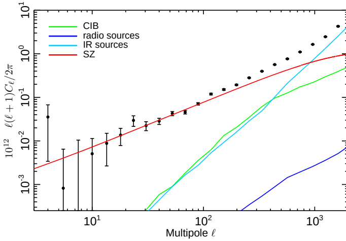
Fig. 15: NILC - MILCA F/L cross-power spectrum (black) compared to the power spectra of the physically motivated foreground models. The considered foregrounds are: clustered CIB (green line); infrared sources (cyan line); and radio sources (blue line). Additionally, the best-fit tSZ power spectrum model presented in Sect. 7.1 is also plotted as a solid red line.
