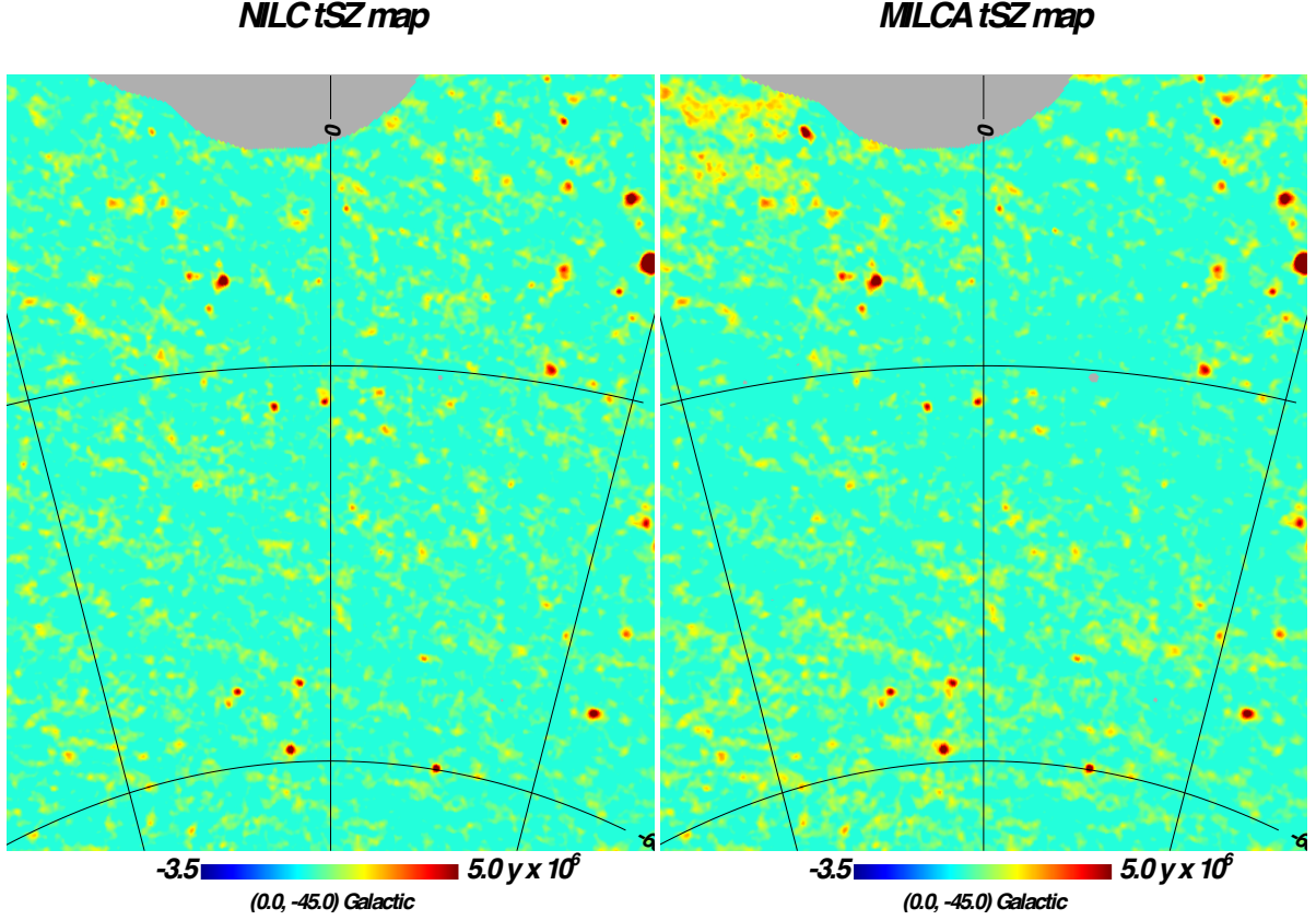
Fig. 3: A small region of the reconstructed Planck all-sky Compton parameter maps for NILC (left) and MILCA (right) at intermediate Galactic latitudes in the southern sky centered at (0, -45) degrees in Galactic coordinates.
