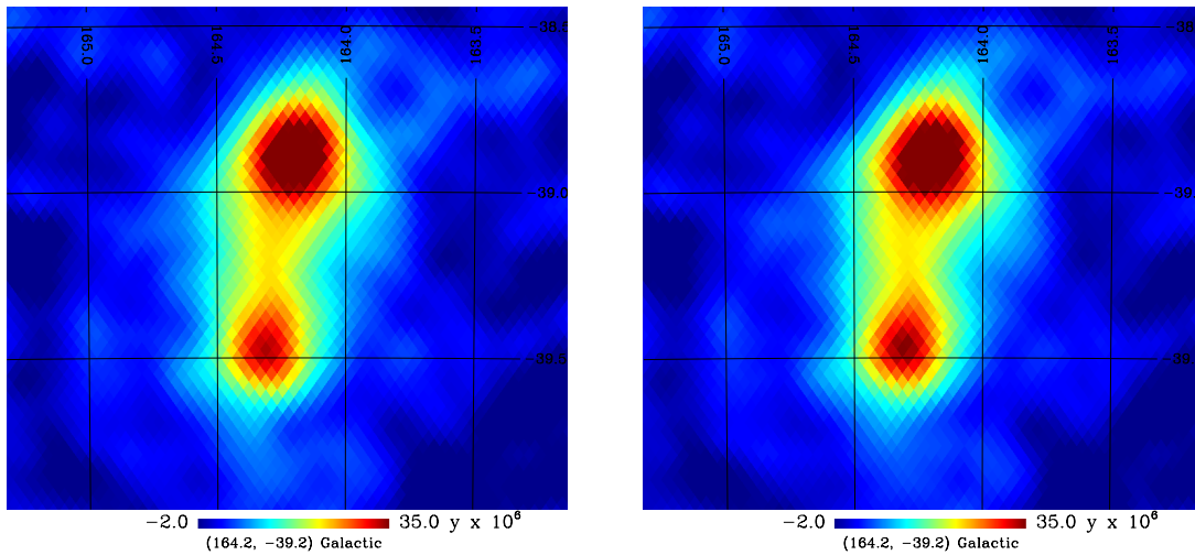
Fig. 8: Compton parameter maps of well known merging systems for MILCA (left column) and for NILC (right column).
