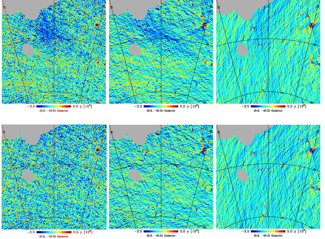
Fig. 4: In and cross scan contributions in the NILC (top line) and MILCA (bottom line) y-maps. From left to right we present the original y-maps, and their in and cross scan contributions for a small region at intermediate Galactic latitudes in the southern sky centered at (0, -45) degrees in Galactic coordinates.
