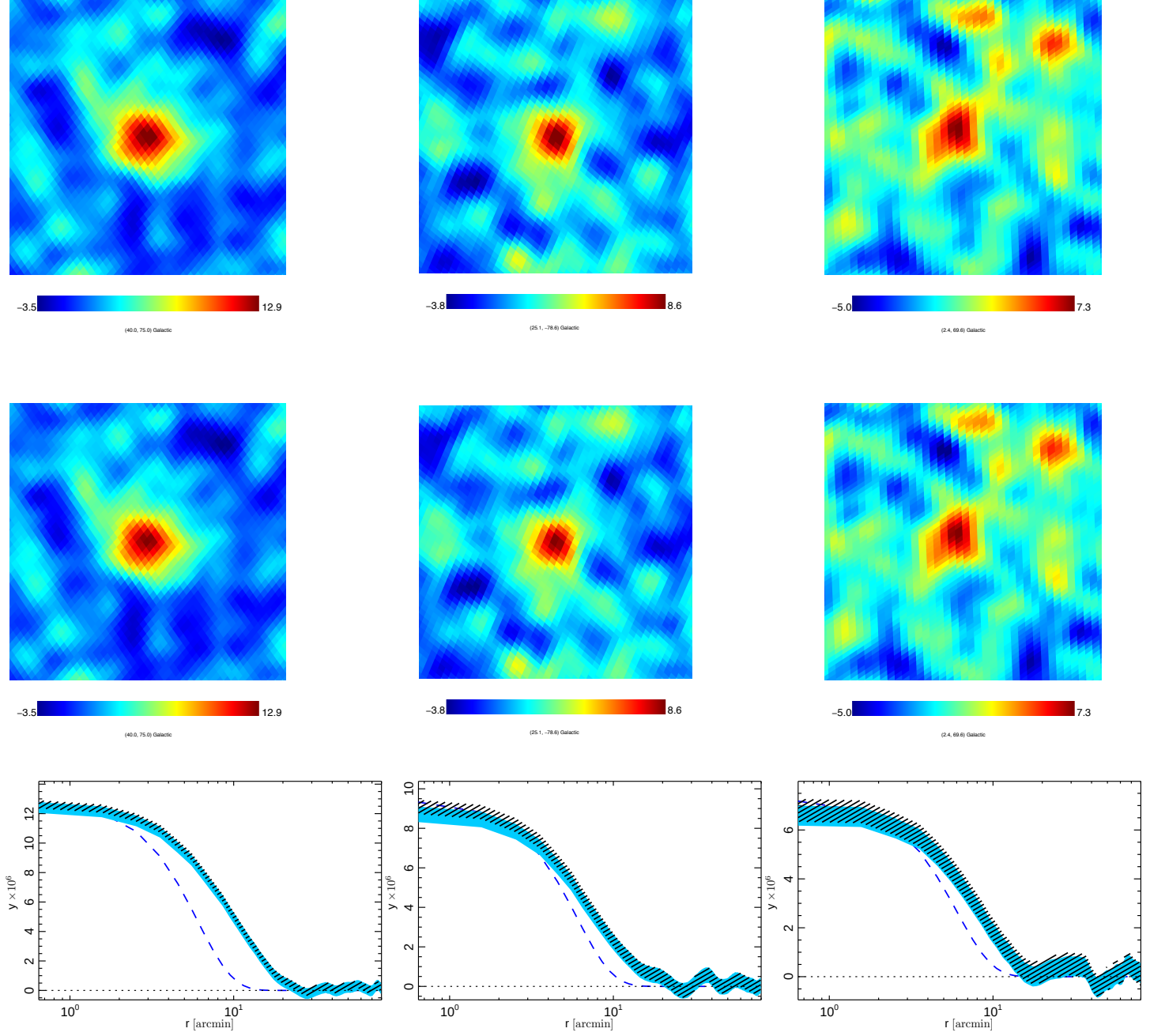
Fig. 7: Compton parameter MILCA (top row) and NILC (middle row) maps for a selection of PSZ2 cluster candidates with signal to noise ratio of 9.3, 6.2 and 4.6 from left to right. The maps are centred at the positions of the clusters in galactic coordinates, which are given at the bottom of the plot. Color scale is in units of y \times 10^{-6} . The bottom row presents the cluster radial profiles for MILCA (black) and NILC (blue). The beam profile is shown as a blue dashed line.
