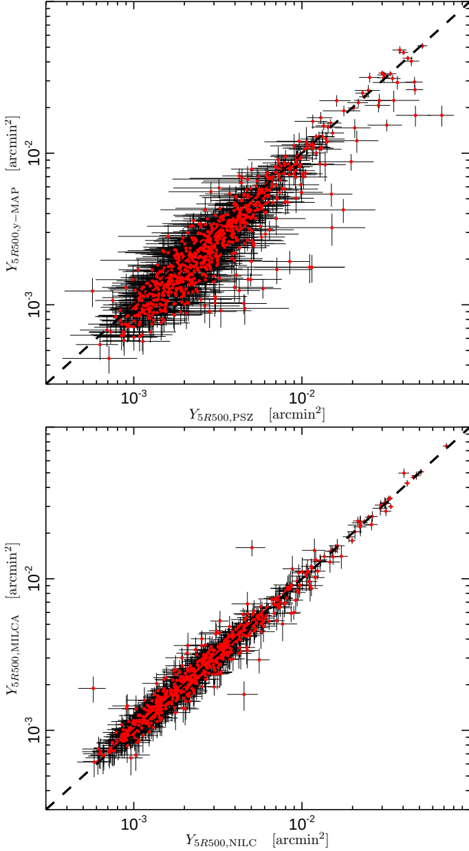
Fig. 6: Top : Comparison between the measured tSZ flux reported in the Planck cluster sample and that estimated directly on the NILC y-map for the blindly detected common sources. Bottom : As above but for the NILC and MILCA measured fluxes.
