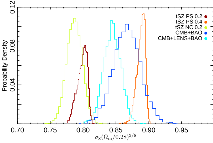
Fig. 19: Marginalised likelihood distribution for \sigma_8(\Omega_m/0.28)^{3/8} for tSZ and CMB based analyses. We represent the tSZ power spectrum analysis results assuming a mass bias, b , of 0.2 (red) and 0.4 (orange), the cluster number count analysis results (green; Planck Collaboration XXIV, 2015 ), and the combined Planck CMB and BAO analysis ( Planck Collaboration XIII, 2015 ) with (cyan) and without (blue) extra lensing constraints.
