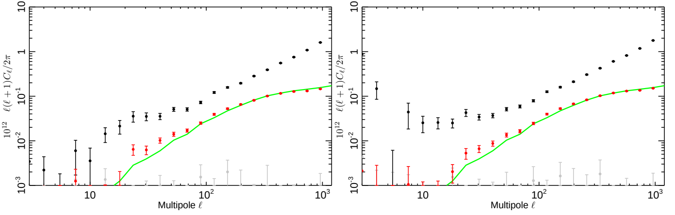
Fig. 12: Comparison of the tSZ angular power spectrum estimated from the cross-power-spectrum of the NILC (left) and MILCA (right) F/L maps (black) with the expected angular power spectrum of the confirmed clusters in the Planck Cluster Sample (green line). The angular cross-power spectrum between the NILCA and MILCA Compton parameter maps and the simulated detected cluster map is shown in red. The correlation between the reconstructed y-map and the simulated detected cluster map, to which an arbitrary rotation has been applied, is plotted in grey.
