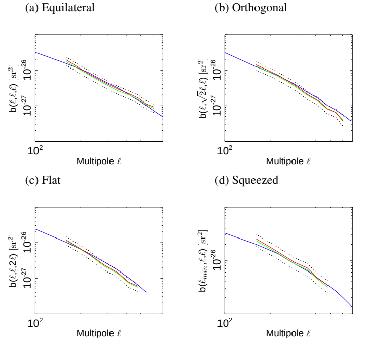
Fig. 14: Bispectra of the NILC (green) and MILCA (red) y-maps for four different configurations (equilateral, orthogonal, flat and squeezed), compared with the bispectrum of the projected map of the PSZ2 clusters (blue). \pm 1\sigma uncertainties are indicated as black dotted lines.
