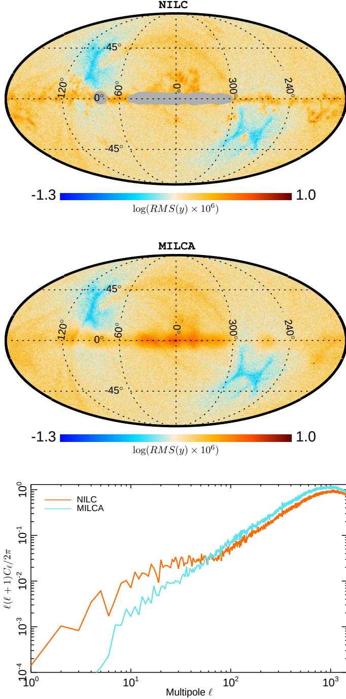
Fig. 5: Top : Standard deviation maps for the NILC (top) and MILCA (middle) y-maps corresponding to the inhomogeneous noise contribution computed from the half difference of the half-rings maps. Bottom : Angular power spectrum of the homogenous noise contribution for the NILC (orange) and MILCA (blue) y-maps (see main text for details).
