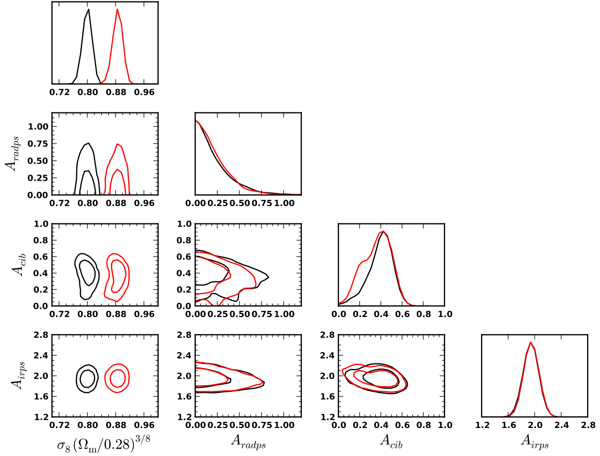
Fig. 16: 2D and 1D likelihood distributions for the combination of cosmological parameters \sigma_8(\Omega_m/0.28)^{3/8} , and for the foreground parameters A_{\text{Rad,PS}} , A_{\text{CIB}} and A_{\text{IR,PS}} . We show the 68.3% and 95.4% C.L. contours. The red and black contours correspond to a fixed mass bias of 0.2 and 0.4 respectively.
