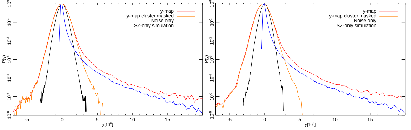
Fig. 13: 1D PDF of the Planck y-map before (red) and after (orange) masking the PSZ2 clusters, and of the half-difference map (black) for the NILC (left) and MILCA (right) methods. We also show for comparison the 1D PDF of the simulated PSZ2 cluster map (dark blue).
