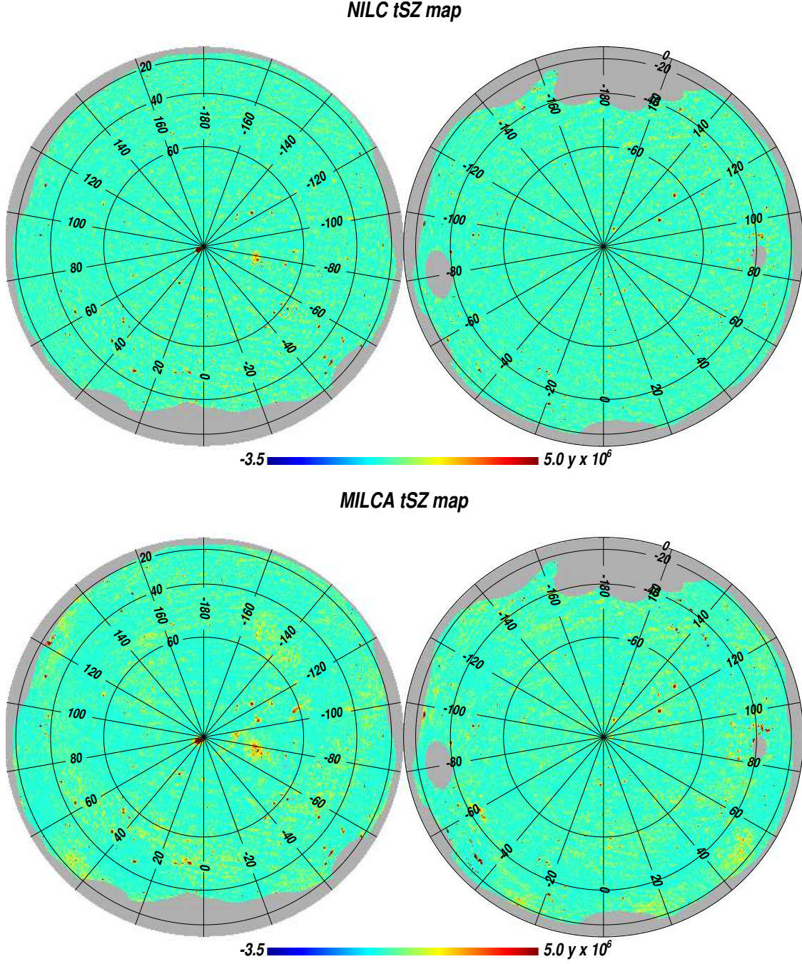
Fig. 2: Reconstructed Planck all-sky Compton parameter maps for NILC ( top ) and MILCA ( bottom ) in orthographic projections. The apparent difference in contrast observed between the NILC and MILCA maps comes from differences in the residual foreground contamination and from the differences in the filtering applied for display purposes to the original Compton parameter maps. For the MILCA method filtering out low multipoles reduces significantly the level of foreground emission in the final y -map. The wavelet basis used in the NILC method was tailored for tSZ extraction. For details see Planck Collaboration XXII (2015) .
