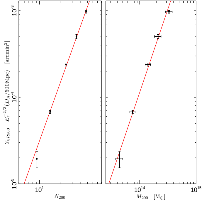
Fig. 10: Integrated tSZ signal as a function of cluster richness (left) and total mass (right). The black points correspond to the average signal obtained for the richness bins considered in Figure 9. The red line represents the corresponding best-fit power law (Eqs. 4 and 6 respectively). Considering z \leq 0.42 , there are 13814 objects for 8 < N_{200} \leq 10 , 37250 for 10 < N_{200} \leq 20 , 7458 for 20 < N_{200} \leq 30 , 2069 for 30 < N_{200} \leq 40 , and 1133 for 40 < N_{200} \leq 60 .
