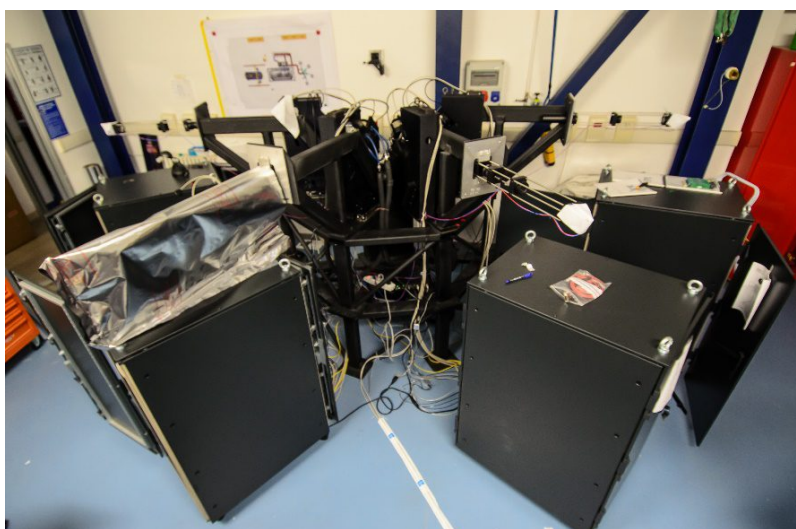
Figure 7 FEU cabinet integration in Merate
