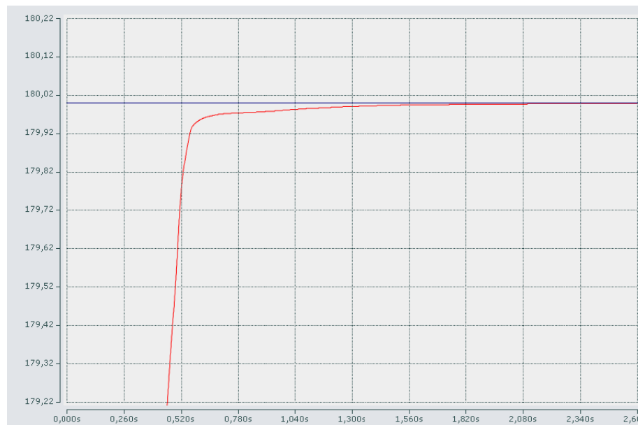
Figure 8 AFW65 Micos rotary stage, positioning detail
