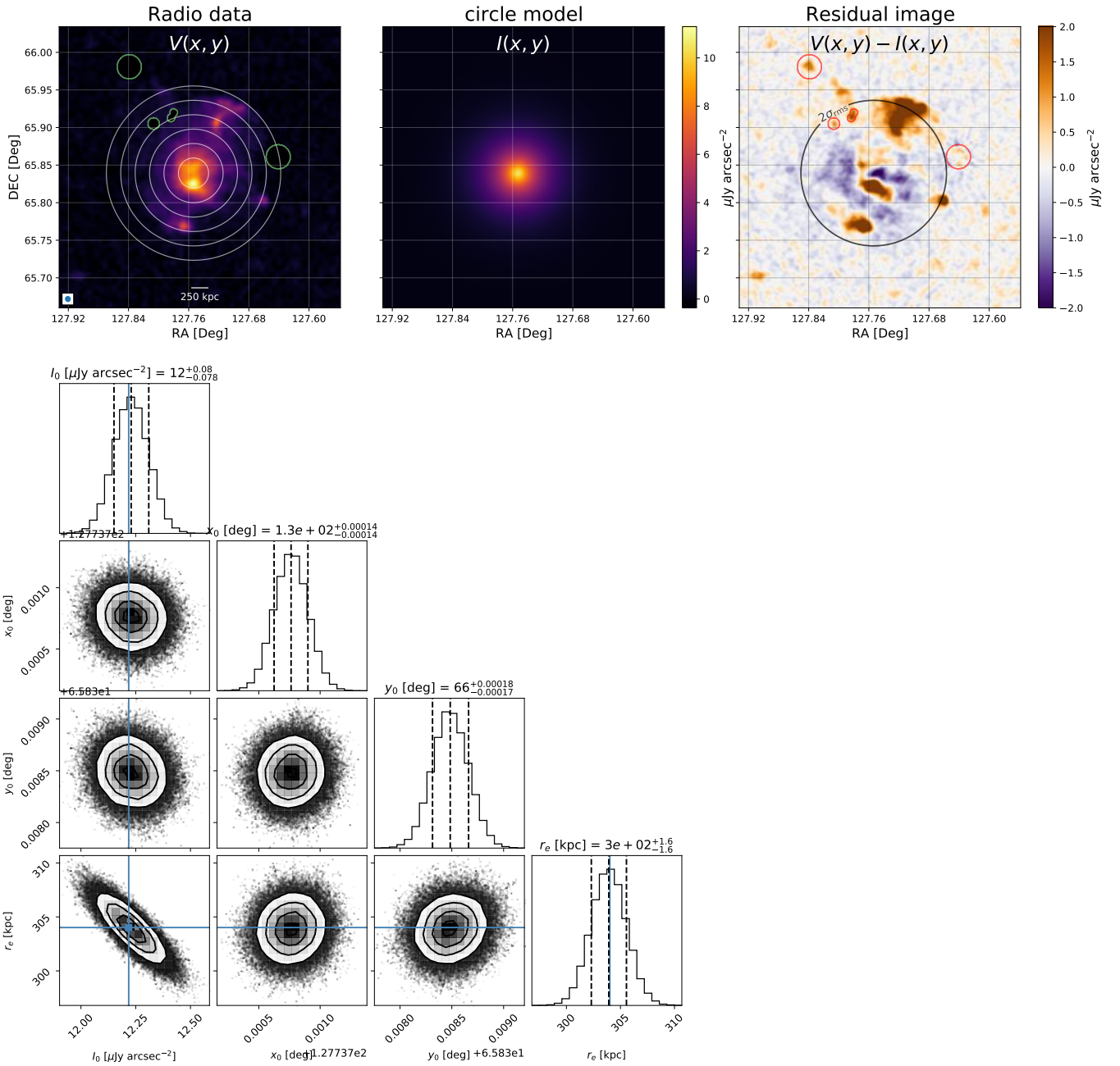
Fig. 6. Results obtained by fitting the radio halo shown in Fig. 3 with HALO-FDCA (Boxelaar et al. 2021). Top figures: image used for the fit with overlaid: the contours (white circles) of the best-fit circular model drawn at [1, 2, 4, 8, \dots] \times \sigma (left panel), the image of the best-fit model (central panel), and the residual image of the fit, with the 2\sigma model contour denoted by the black circle (right panel). Contaminating sources are masked out and are highlighted by the green and red regions (left and right panels, respectively). Bottom figure: MCMC corner plot presenting the distribution of the posteriors of each fitted parameter (Foreman-Mackey et al. 2013).
