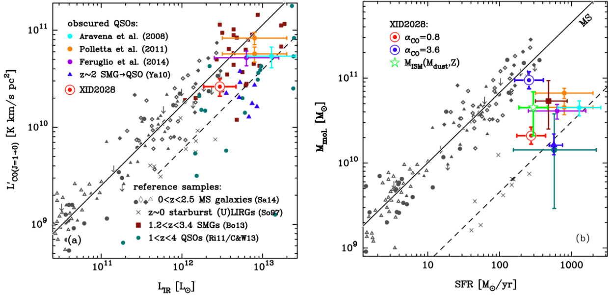
Fig. 3. Left panel: L'(\text{CO}[1-0]) against the IR luminosity ( 8-1000\ \mu\text{m} ) showing a compilation of MS galaxies at 0 < z < 2.5 from the Sargent et al. (2014) work (Sa14; grey symbols), local ULIRGs from from So97, crosses SMGs from Bothwell et al. (2013; Bo13, filled brown squares), 1 < z < 4 QSOs with data from Riechers (2011) and Carilli & Walter (2013; R11/C&W13, light blue circles). The measurement for XID2028 obtained assuming r_{31} = 0.7 is shown as a red circle. Obscured QSOs proposed to be in the transition phase presented in Aravena et al. (2008), Polletta et al. (2011), Feruglio et al. (2014) and the MIPS-selected sources from Yan et al. (2010) are also marked, as labelled. Right panel: inverse, integrated Kennicutt-Schmidt relation between SFR and molecular gas mass. The colour points correspond to the position of XID2028 with different CO-to- \text{H}_2 conversion factors: \alpha_{\text{CO}} = 3.6 (top; blue), and \alpha_{\text{CO}} = 0.8 (bottom; red). The green star shows the ISM mass inferred from the dust SED. All the values for XID2028 are slightly offset in the x-axis for clarity. Other points are taken from the same samples presented in the left panel. For the Bo13, R11/C&W13, and Ya10 samples we plot the median value with associated 16% and 84% percentiles. For the obscured QSOs all the authors used \alpha_{\text{CO}} = 0.8 . In both panels, the solid black line is the best-fit relation for MS galaxies, and the dashed line defines the locus of strong SB galaxies with approximately 15 times shorter depletion time ( M_{\text{mol}}/\text{SFR} ) than MS galaxies (Sargent et al. 2014).
