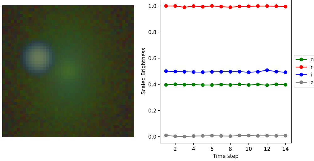
Figure 11: A negative example on the LSST-wide data set – This datum belongs to the “LSNCC” class, but has been classified as “Lens”. The lensing effect is alluded by the halo surrounding the star, while the flat time series suggests the absence of a transient phenomenon, which induces the wrong classification
