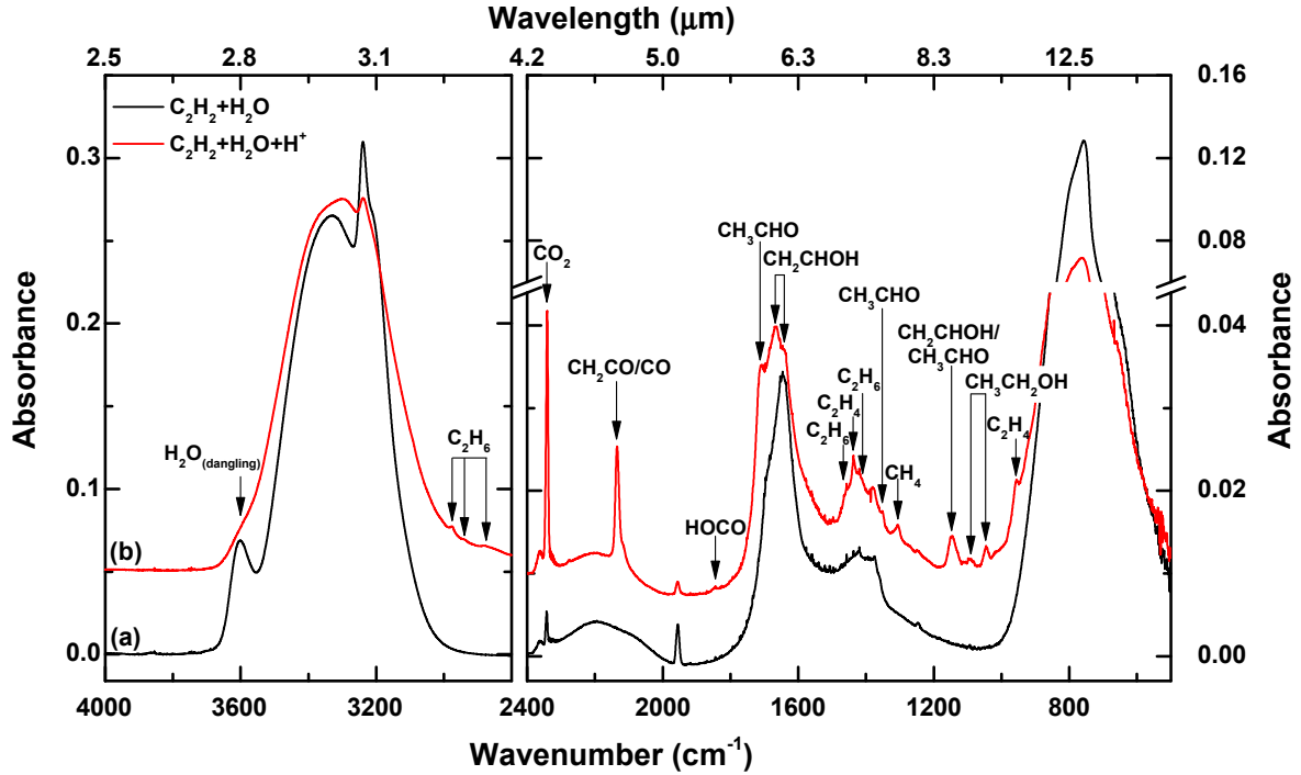
Fig. 1. IR spectra obtained after (a, black) deposition of \text{C}_2\text{H}_2:\text{H}_2\text{O} mixed ice and (b, red) following ion radiolysis by 200 keV \text{H}^+ at 17 K. The initial deposition ratio of \text{C}_2\text{H}_2:\text{H}_2\text{O} mixed ice was 0.4:1, and the applied \text{H}^+ fluence was 6.0 \times 10^{14} protons \text{cm}^{-2} . IR spectra are offset for clarity.
