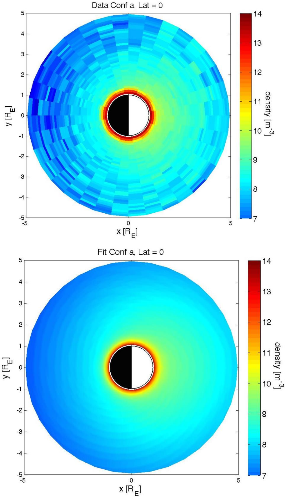
Figure 4 Above: Monte Carlo simulated equatorial exosphere of O_2 generated after O^+ impacts in the configuration a of P2013: leading corresponding to the illuminated side + x direction, Jupiter facing hemisphere in + y direction. Below: density ( O_2 after O^+ ) obtained by 2D fit in the equatorial plane
