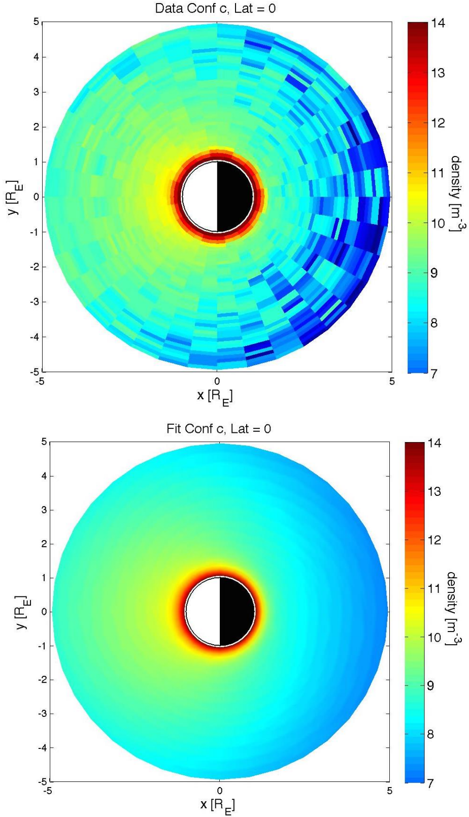
Figure 6 Same as Figure 4 for Conf c. Above: Monte Carlo simulated equatorial exosphere of \text{O}_2 generated after \text{O}^+ impacts in the configuration c of P2013. Below: density ( \text{O}_2 after \text{O}^+ ) obtained by 2D fit in the equatorial plane
