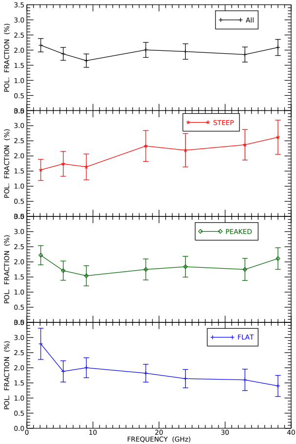
Figure 4. Median polarization fraction behaviour with frequency (at 2.1, 5.5, 9, 18, 24, 33 and 38 GHz) for all the sources (black), for steep sources (red), for peaked (green) and flat ones (blue). The errors on median values are given by 1.253 \times \text{rms}/\sqrt{N} , where rms is the standard deviation around the mean and N is the number of the data (at a given frequency) for a given class of objects (cf. Arkin & Colton 1970).
