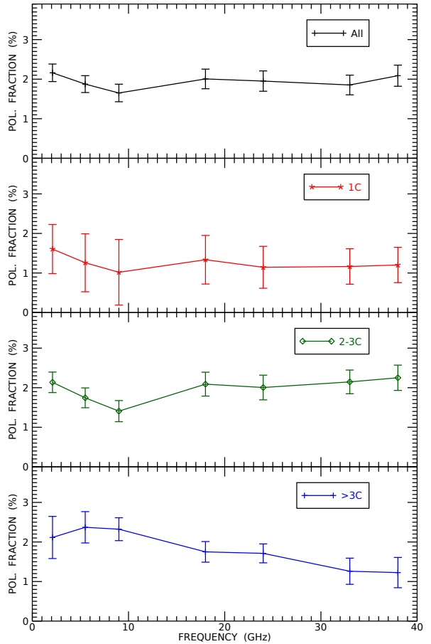
Figure 5. Median polarization fraction at the observation frequencies (2.1, 5.5, 9, 18, 24, 33 and 38 GHz) for all the sources (black), for '1C' sources (red), for '2-3C' sources (green) and for sources with more than 3 components (blue, labelled '>3C'). The errors on median values are given by 1.253 \times \text{rms}/\sqrt{N} , where rms is the standard deviation around the mean and N is the number of detected sources (cf. Arkin & Colton 1970).
