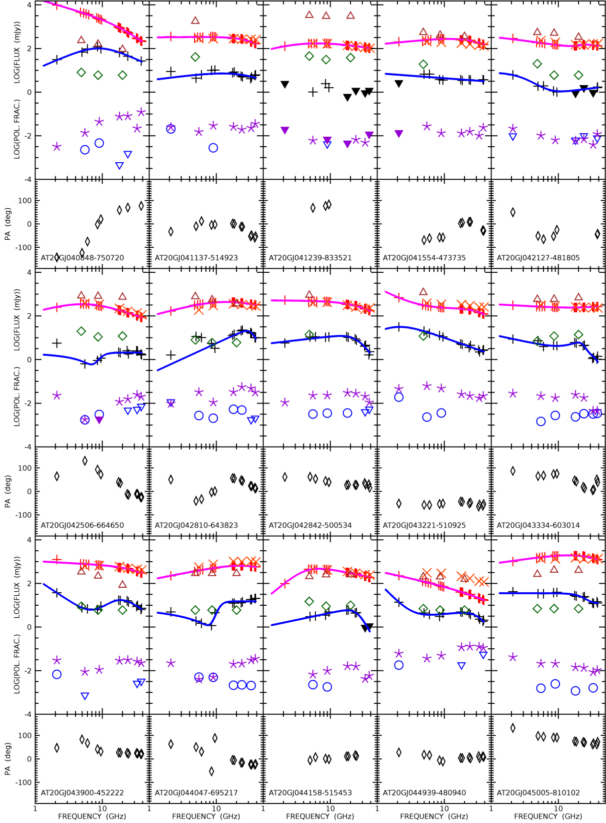
Figure 1. ( Continued. ) Other quantities available only for the September 2014 and March-April 2016 campaigns: linear polarization fractions: purple asterisks with upper limits shown as downwards pointing purple filled triangles; circular polarization fraction: violet circles and downward triangles for upper limits. Polarization angle (PA): black diamonds.
