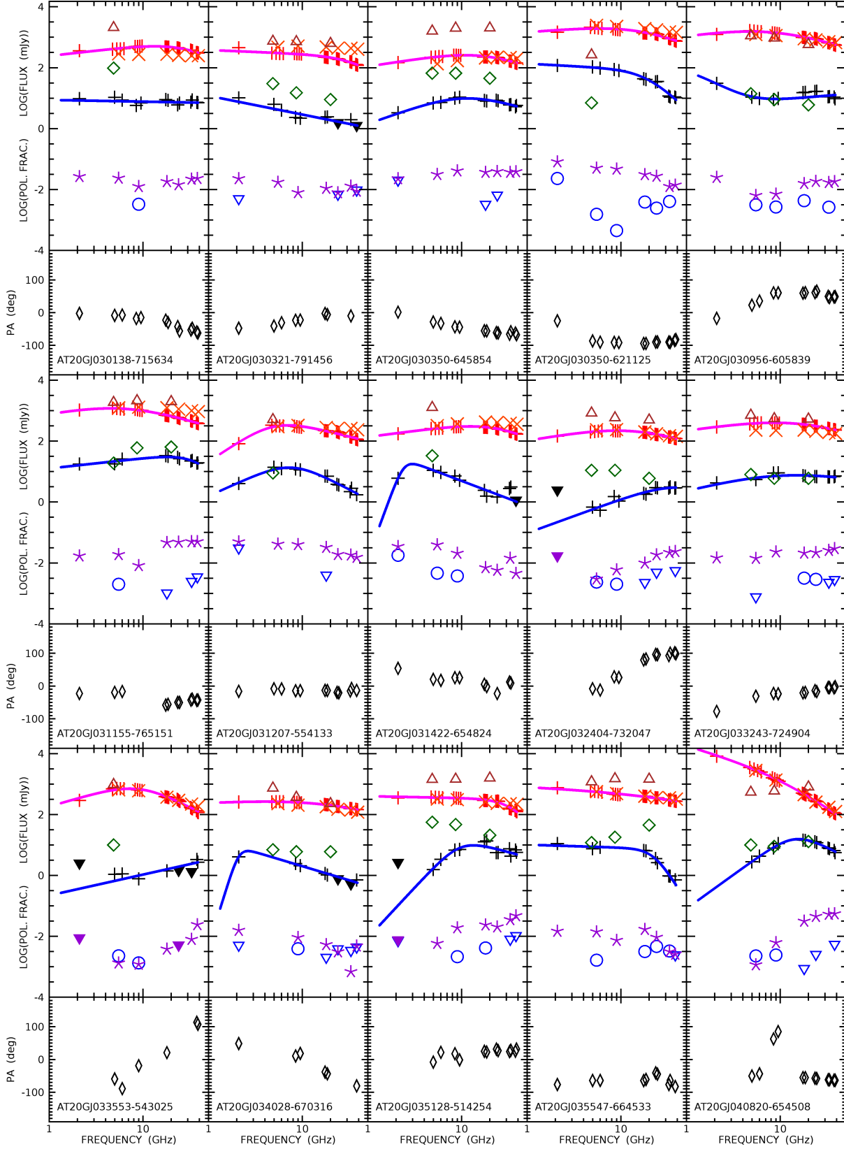
Figure 1. Spectra in total intensity and polarization, polarization fraction and polarization angle for the 107 objects of the faint PACO sample, observed in the September 2014 and March-April 2016 campaigns. The error bars are not displayed since they are smaller than the symbols. Total intensity: red pluses indicate our observations and the solid magenta lines show the fitting curves. The orange crosses show the median PACO flux densities (July 2009-August 2010) while the brown triangles represent the AT20G observations (best epoch in 2004-2008). Polarization (flux density): black pluses refer our observations. Upper limits are shown as black filled downwards triangles. The solid blue lines indicate the best fit curves. The AT20G observations (best epoch in 2004-2008) are represented by green diamonds. ( Continued... )
