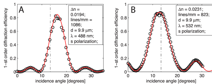
Fig. 7. Efficiency measurements at fixed wavelength (s-polarized), fitted with RCWA, for the two VPHGs composing the GRISMs for the spectrograph ALFOSC; A) is the BLUE grating, B) is the GREEN grating. Inside the inlets are reported the calculated values of refractive index modulation. The vertical dotted lines indicate the angle at which the gratings work in the GRISM configuration. The light is deviated by the prisms and enters the VPHGs at 13.4^\circ .
