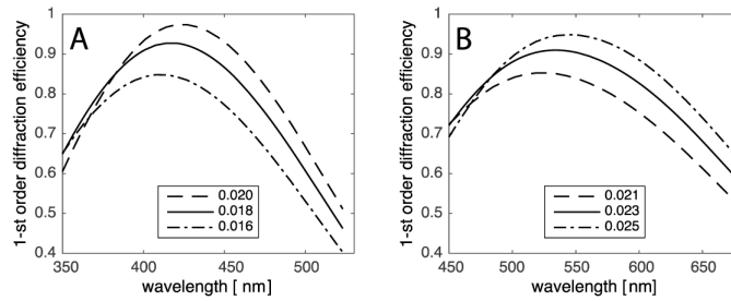
Fig. 6. RCWA simulations with different refractive index modulation values (reported in the legend) for a 10 \mu\text{m} thick grating and an incidence angle of 13.4^\circ . A) Wavelength range for the BLUE device (1080 l/mm); B) wavelength range for the GREEN device (820 l/mm).
