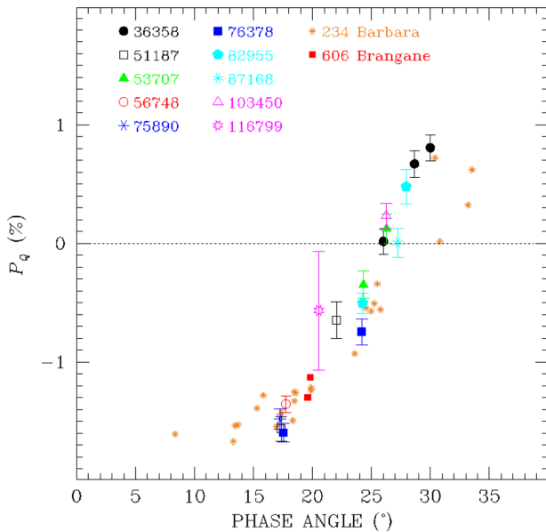
Figure 3. Polarization versus phase angle data for the targets of the present investigations, as well as a couple of measurements of (606) Brangane, the largest member of the family, previously observed at the Calern observatory. The family data are compared with the polarization curve of the prototype of Barbarians, (234) Barbara, whose available measurements are shown, for sake of clarity, without their associated error bars (orange symbols).
