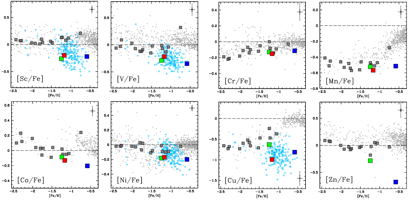
Fig. 4. Iron-peak elements' abundance ratios as a function of [Fe/H] , for SMC and MW GCs and field stars (same symbols and data as in Fig. 3). MW field stars data are from Fulbright (2000), Stephens & Boesgaard (2002), Gratton et al. (2003), Reddy et al. (2003, 2006), Bensby et al. (2005), Adibekyan et al. (2012), Roederer & Lawler (2012) and Reggiani et al. (2017).
