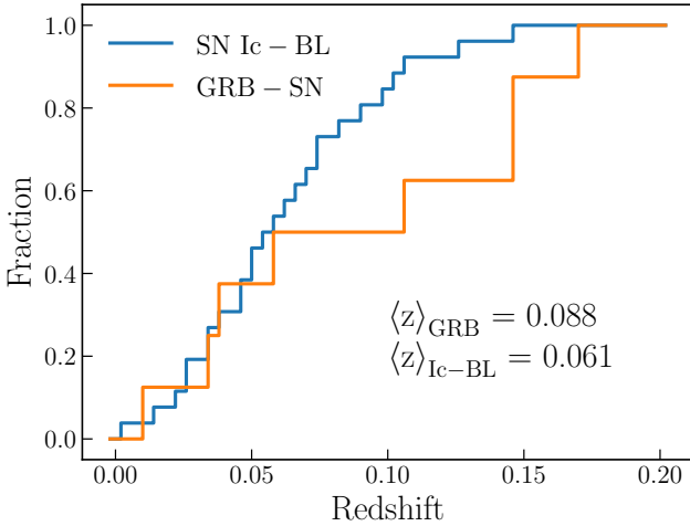
Fig. 2. Cumulative redshift distributions of the GRB-SN and SN Ic-BL samples. Indicated are mean redshifts of the distributions.
