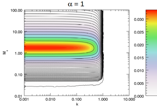
Figure 10. Distribution of the growth rate, -\text{Im}(\omega) , of the toroidal buoyancy mode as a function of the wavenumber k and M_a for \gamma_c = 1.01 , \alpha = 1 and P_c = 1 .
