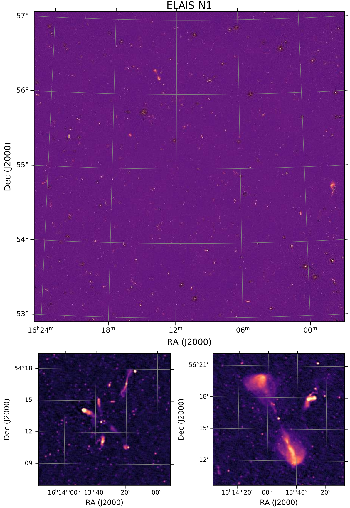
Fig. 2. Final deep image of the central region of ELAIS-N1 field. Top panel: a wide-field view containing about one third of the total area. Lower panels: zoomed-in regions (each around 0.1 per cent of the full image area), showing the high image quality for extended sources and sensitivity to faint sources. All images are Stokes I , with 6 arcsecs resolution. The full-field image contains more than 85 000 sources.
