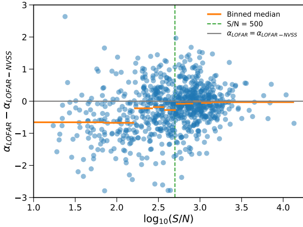
Fig. 16. Difference between the intra-band spectral index ( \alpha_{\text{LOFAR}} ) and the NVSS spectral index ( \alpha_{\text{LOFAR-NVSS}} ) compared to the S/N of the cross-matched sources. The distribution of S/N is divided in deciles and the median of the difference is computed and shown as orange lines. The spectral indices are flatter (lower values of the difference) for low S/N likely due to incompleteness effects. The distribution is close to zero (marked as a horizontal grey line) for sources with S/N > 500 (shown as a vertical green dashed line).
