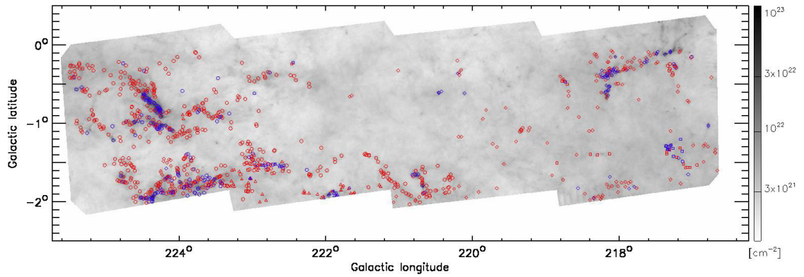
Figure 3: Spatial distribution of the Hi-GAL compact sources (surviving the filtering of the band-merged catalogue), overplotted on the column density map of the same field shown in Figure 1 (details about the derivation of the column density map can be found in [7]). The blue and red colors indicate protostellar and starless sources, respectively.
