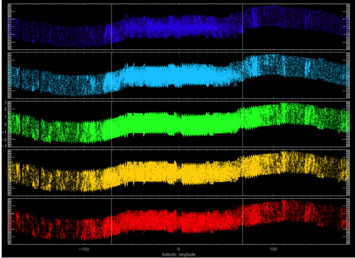
Figure 2: Distribution in the [\ell, b] plane of the Hi-GAL compact sources detected in single bands by [3]. From top to bottom: 70\ \mu\text{m} (blue dots), 160\ \mu\text{m} (cyan), 250\ \mu\text{m} (green), 350\ \mu\text{m} (yellow), 500\ \mu\text{m} (red).
