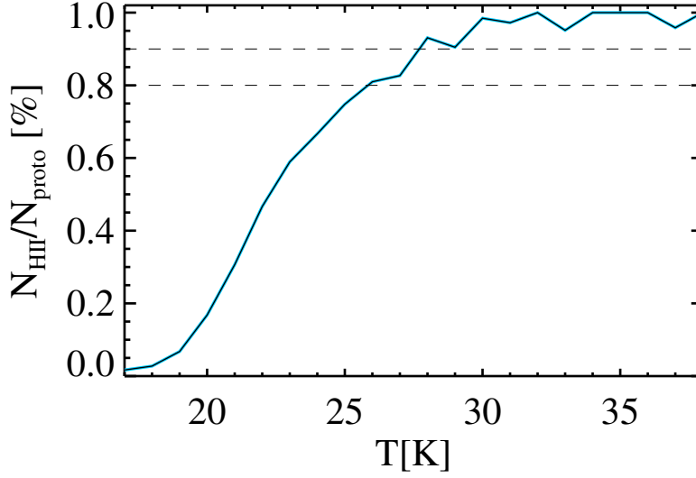
Figure 5: Fraction of protostellar sources classified as HII-region candidates (based on their L_{\text{bol}}/M ratio) over the total number of the protostellar ones vs temperature. The two horizontal dashed lines indicate the 80% and 90% levels.
