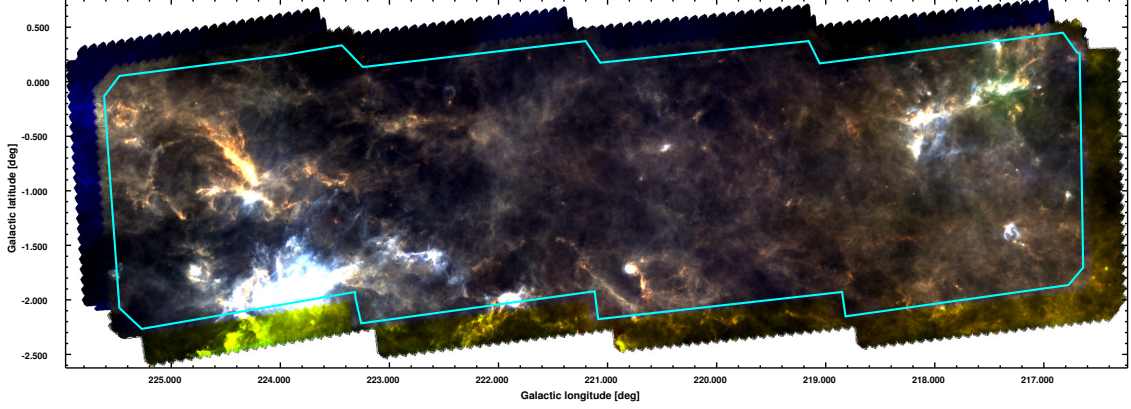
Figure 1: Example of Hi-GAL maps: RGB composite of the 216.^{\circ}5 < \ell < 225.^{\circ}5 Hi-GAL field (blue: PACS 160\ \mu\text{m} ; green: SPIRE 250\ \mu\text{m} ; red: SPIRE 500\ \mu\text{m} ), from [7]. The color scaling is linear. The cyan contour delimits the common science area covered by both PACS and SPIRE.
