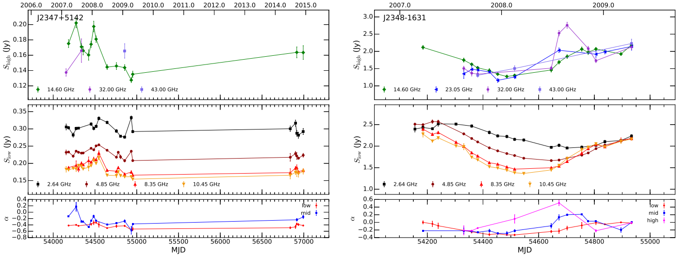
Fig. B.18. Multi-frequency light curves for all the sources monitored by the F-GAMMA programme (“f”, “s1”, “s2”, “old”) and the F-GAMMA- Planck MoU. The lower panel in each frame shows the evolution of the low (2.64, 4.85 and 8.35 GHz) and mid-band (8.35, 10.45 and 14.6 GHz) and high-band (14.6, 23.05, 32, 43 GHz) spectral index. Only spectral index estimates from at least three frequencies are shown. Connecting lines have been used to guide the eye.
