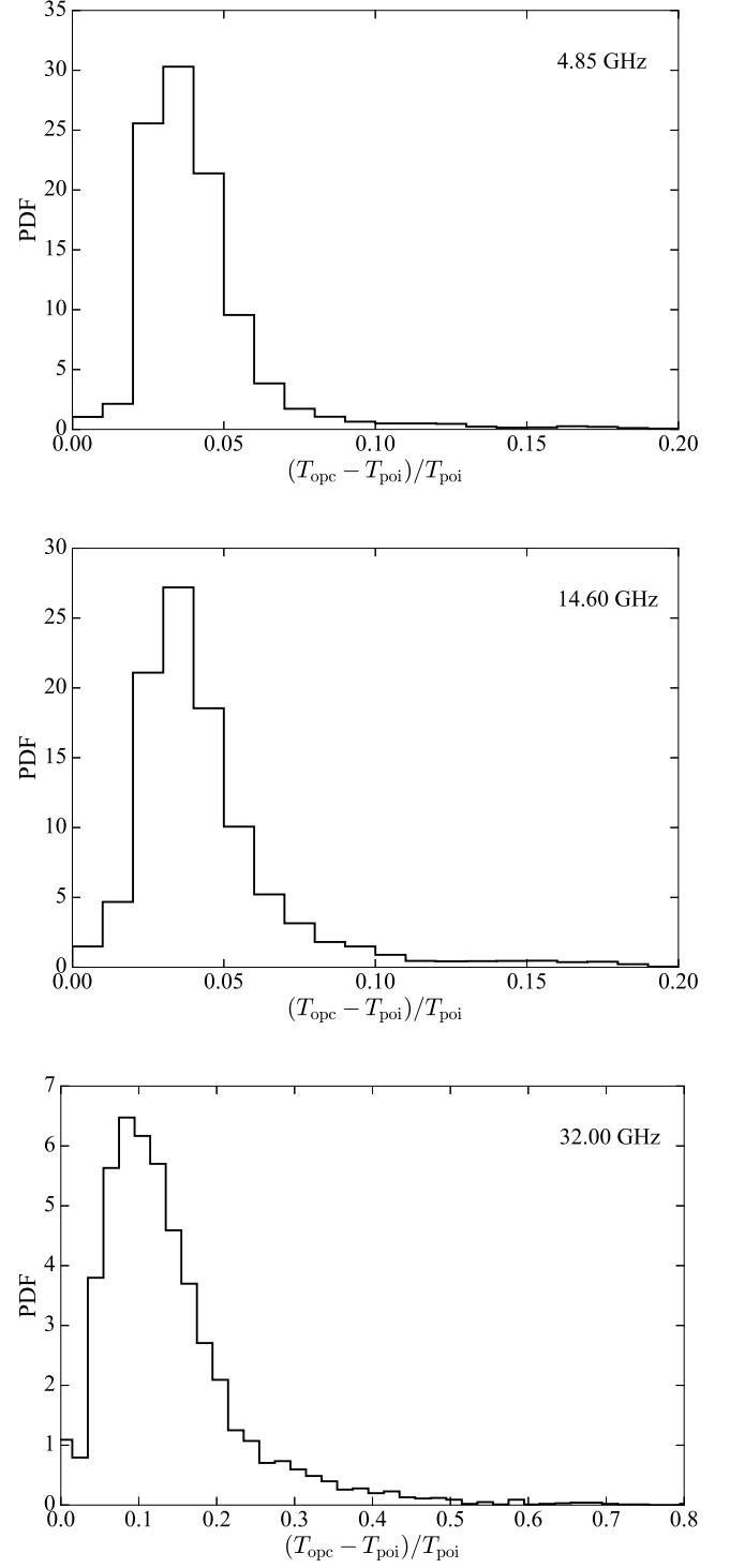
Fig. 5. Fractional opacity correction. Upper panel: 4.85 GHz (low band), middle panel 14.60 GHz (intermediate band), and lower panel 32.00 GHz (high band). The x-axis is the fractional increase of the antenna temperature corrected for pointing ( T_{\text{poi}} ) after the opacity correction has been applied ( T_{\text{opc}} ).
