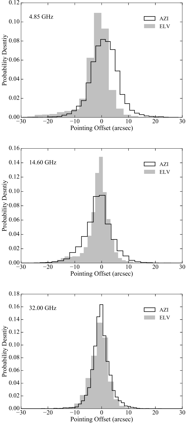
Fig. 3. Pointing offsets for scans that have passed basic quality checks. Upper panel: 4.85 GHz (low band), middle band panel 14.60 GHz (intermediate band), and lower panel 32.00 GHz (high band). The black solid line corresponds to the longitudinal scan and the grey area to the latitudinal scan.
