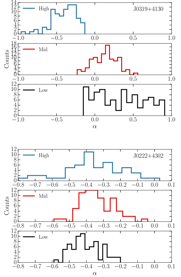
Fig. 10. Spectral index distribution in three sub-bands. Upper panel: a source undergoing intense spectral evolution. Lower panel: a source with an almost self-similarly variable SED.
