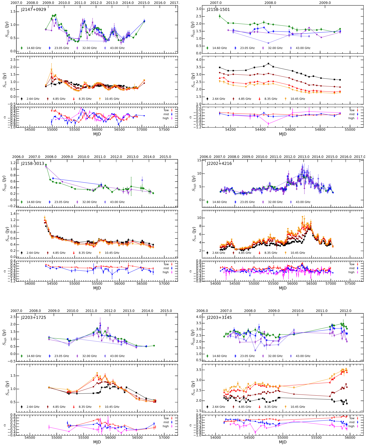
Fig. B.16. Multi-frequency light curves for all the sources monitored by the F-GAMMA programme (“f”, “s1”, “s2”, “old”) and the F-GAMMA-Planck MoU. The lower panel in each frame shows the evolution of the low (2.64, 4.85 and 8.35 GHz) and mid-band (8.35, 10.45 and 14.6 GHz) and high-band (14.6, 23.05, 32, 43 GHz) spectral index. Only spectral index estimates from at least three frequencies are shown. Connecting lines have been used to guide the eye.
