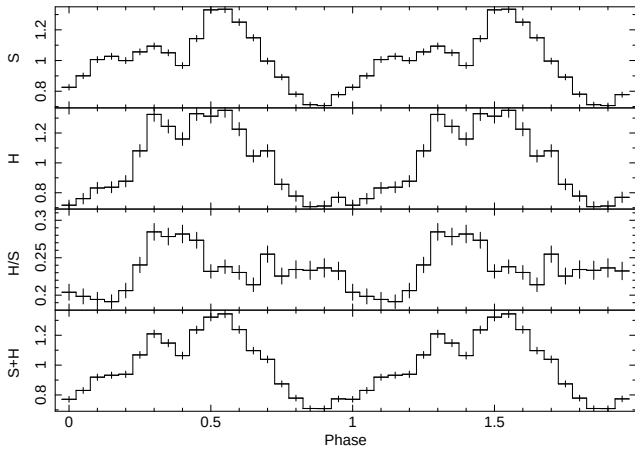
Fig. 4. IGR J11215–5952 pulse profile folded on the spin period of 187 s, assuming MJD 57432 as epoch of phase zero. The whole NuSTAR exposure time has been considered. From top to bottom: soft profile ( S = 3\text{--}12\text{ keV} ), hard one ( H = 12\text{--}78\text{ keV} ), their hardness ratio ( H/S ) and profile in the total band ( S+H = 3\text{--}78\text{ keV} ), respectively. Each pulse profile has been normalised by dividing by the average source intensity in the considered energy band.
