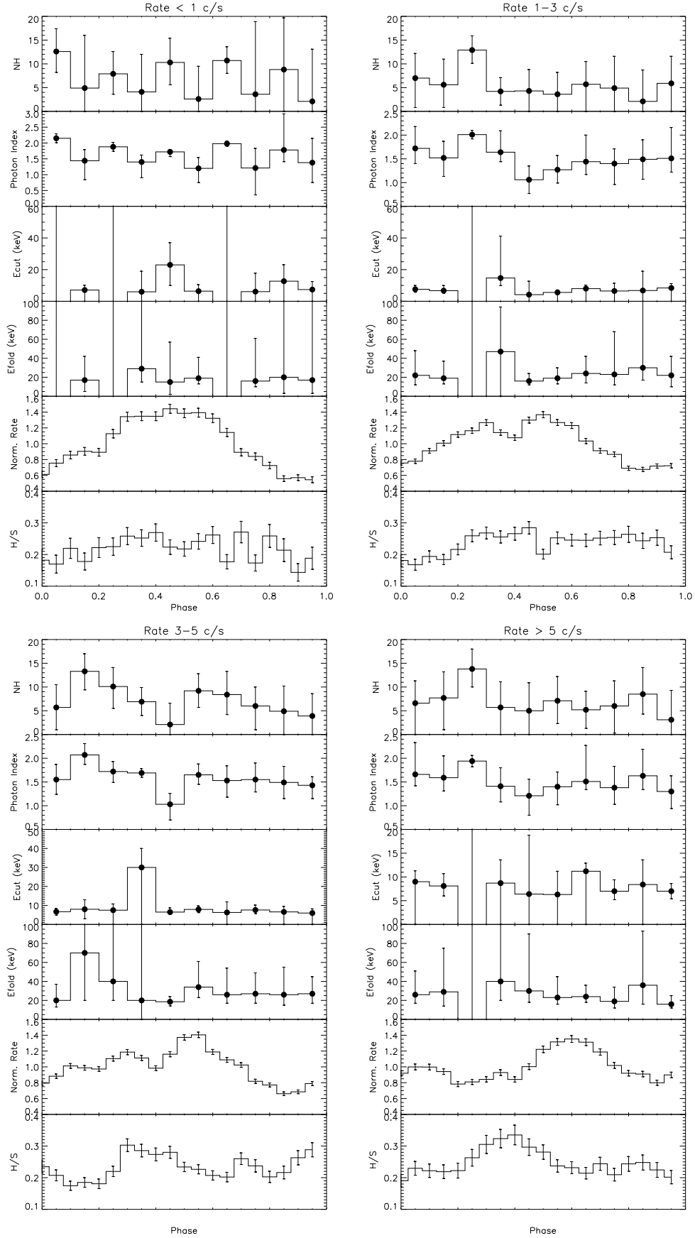
Fig. 9. Spin-phase-selected spectroscopy in four intensity states, as reported in Table 5: from top to bottom, from left to right, the intensity states are below 1 count s -1 , 1–3 count s -1 , 3–5 count s -1 , and above 5 count s -1 . Bottom panels: the intensity-selected pulse profiles (3–78 keV) are reported, together with the hardness ratio (H/S) of hard pulse profile ( H = 12\text{--}78 keV) to the soft pulse profile ( S = 3\text{--}12 keV).
