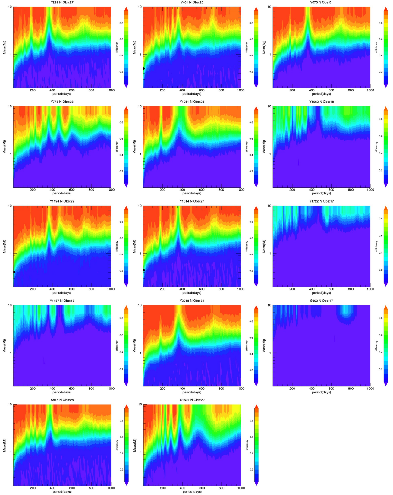
Fig. A.1. Contours of the planet detection efficiency for the MS stars in the domains of 1–1000 days for planet period and 0.2\text{--}10 M_J for planet mass. A 0.01 FAP level has been used as detection planet threshold in the periodogram analysis. A filled circle indicates the planet position.
