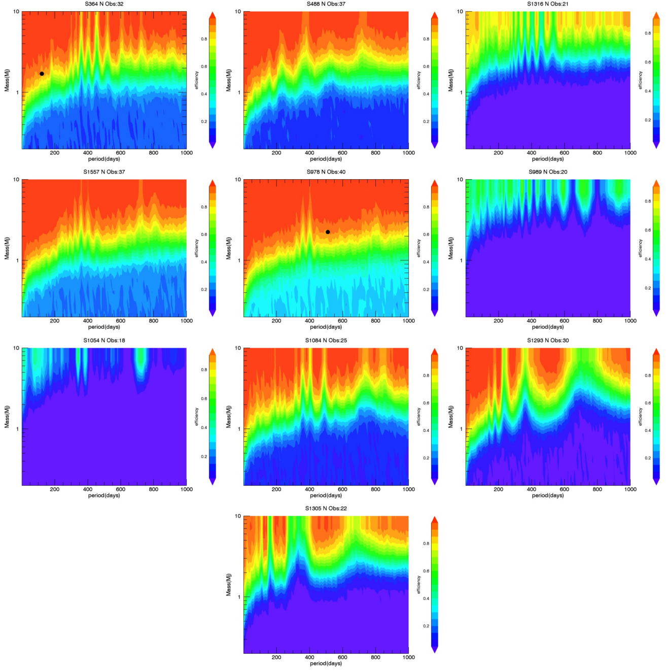
Fig. A.2. Contours of the planet detection efficiency for the evolved stars in the domains of 1–1000 days for planet period and 0.2\text{--}10\ M_J for planet mass. A 0.01 FAP level has been used as detection planet threshold in the periodogram analysis. A filled circle indicates the planet position.
