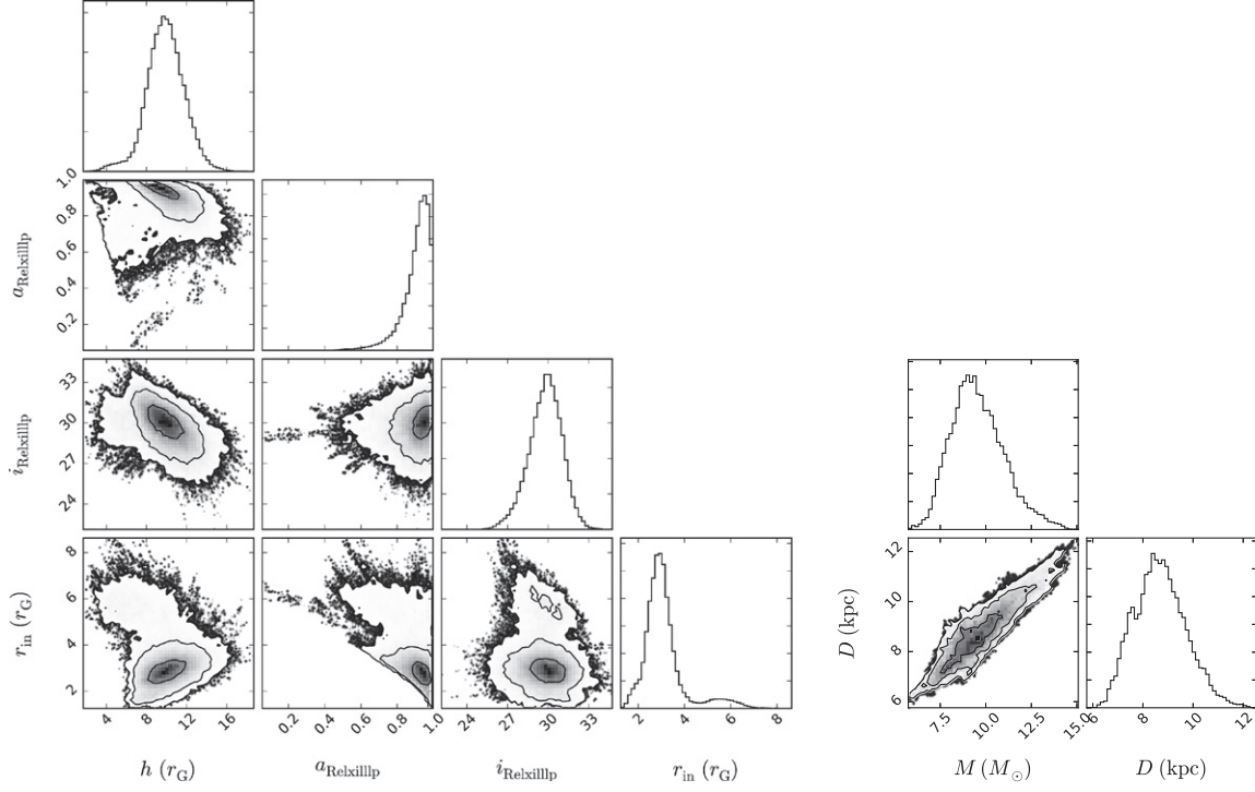
Figure 3. Left: 1, 2, and 3\sigma confidence contours for spin, inclination, source height, and inner disk radius measured using reflection spectroscopy. Source height and inner disk radius are required to be \geq r_{\text{ISCO}} . Right: contours for the mass and distance measured using continuum fitting.
