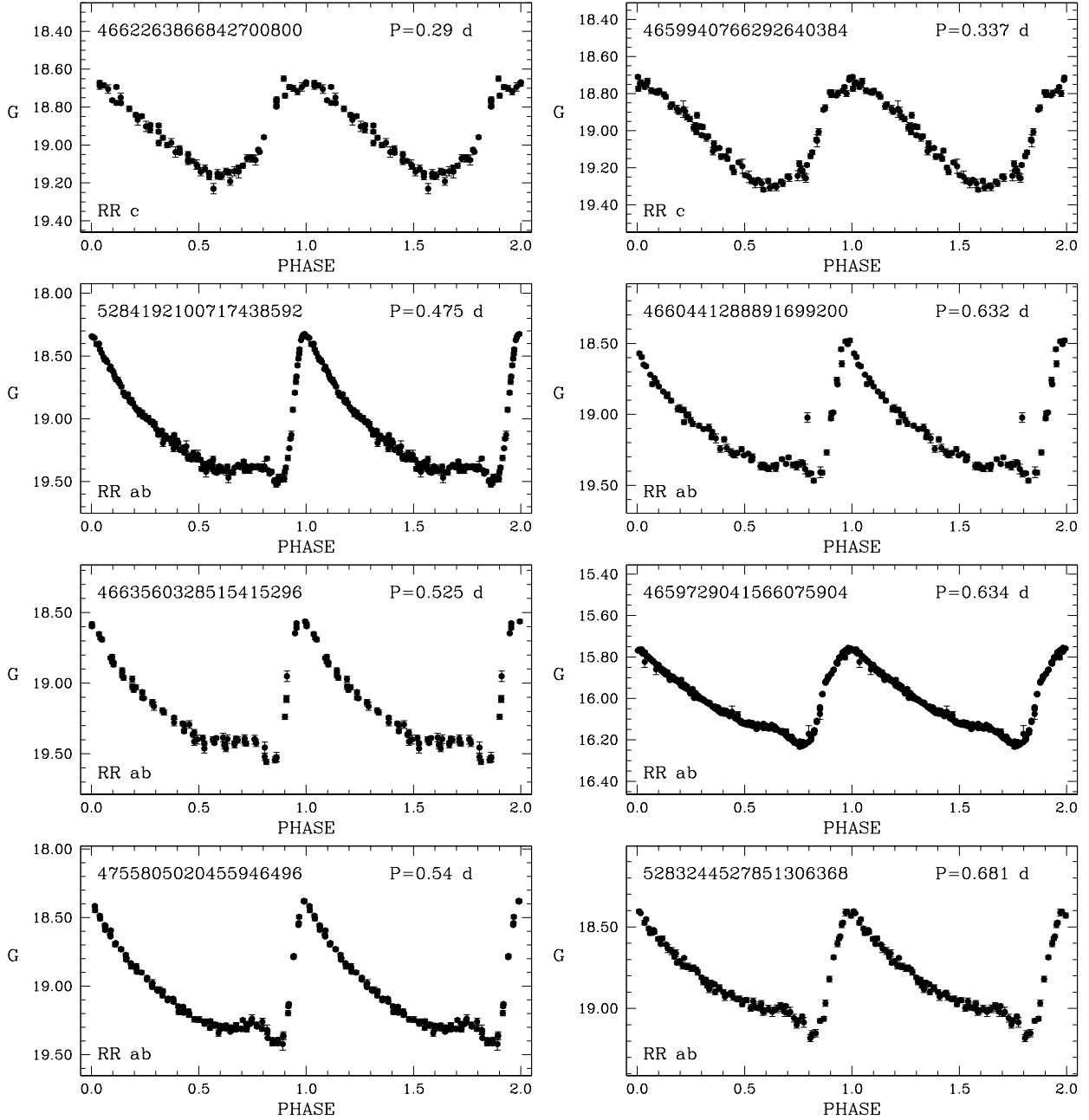
Fig. 23. Examples of G -band light curves of RRc ( top two panels ) and RRAb stars in the LMC and in the MW halo ( third panel on the right ). Typical errors of individual measures at the magnitude level of the LMC RR Lyrae stars are of the order of \gtrsim 0.02 mag. A few measurements with errors larger than 0.05 mag are not displayed.
