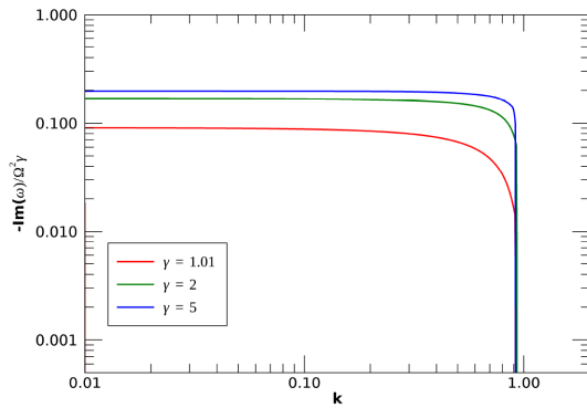
Figure 11. Growth rate of the toroidal mode as a function of k for \alpha = 1 , P_c = 1 , and \gamma_c = 1.01, 2, 5 . The growth rate is normalized by \gamma_c \Omega_c^2 . The three different curves refer to three different values of \gamma_c as indicated in the legend. M_a is also different for the three curves and for each curve it has the value at which the maximum growth rate is reached at a fixed k : M_a = 1.5, 4.5, 15 , respectively, for \gamma_c = 1.01, 2, 5 .
