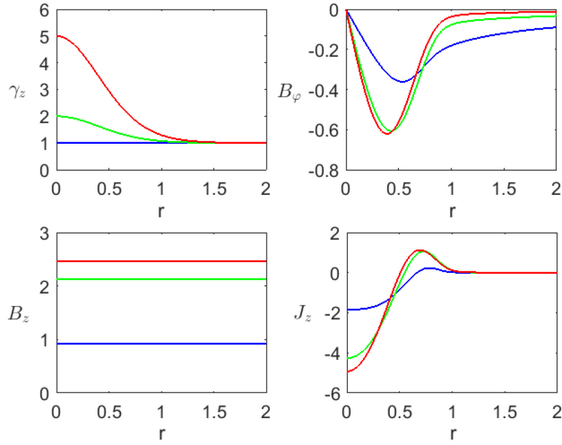
Figure 1. Radial profiles of the Lorentz factor, magnetic field components, and axial current density for the equilibrium at \alpha = 1 , M_a^2 = 1 , P_c = 1 and different \gamma_c = 1.01 (blue), 2 (green), 5 (red).
