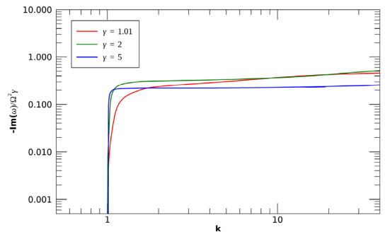
Figure 14. Growth rate of the poloidal buoyancy mode as a function of k for \alpha = 1 , P = 1 , and \gamma_c = 1.01, 2, 5 . The growth rate is normalized by \gamma_c \Omega_c^2 . The three different curves refer to three different values of \gamma_c as indicated in the legend. M_a is different for the three curves and for each curve has the value at which the maximum growth rate is found at fixed k : M_a = 1.8, 5.72, 14.2 , respectively, for \gamma_c = 1.01, 2, 5 .
