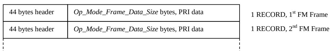
Figure 2.6.5 - 4: Scheme of the Uncompressed data frame structure.
