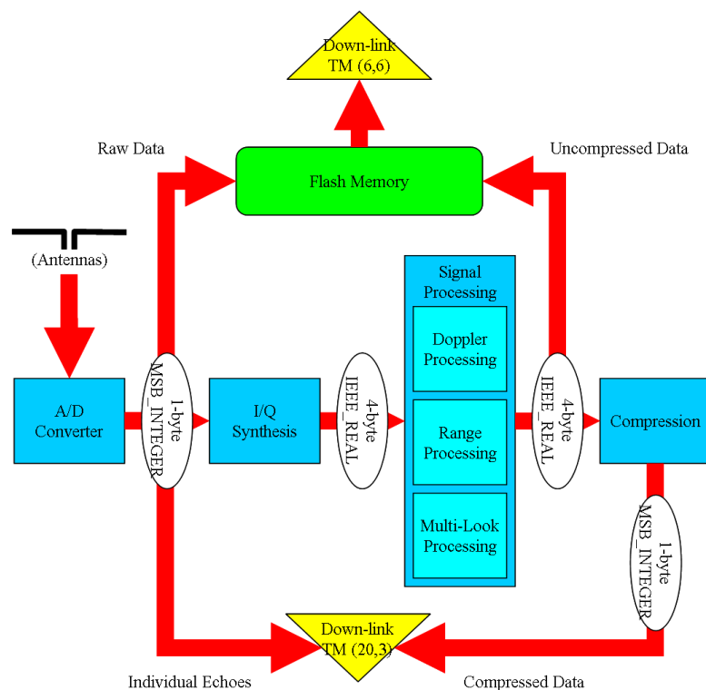
Figure 2.3.8 – 1 Conceptual diagram of MARSIS on-board processing during subsurface sounding. TM (20,3) is the normal scientific telemetry produced by the instrument during operation, while TM (6,6) is the telemetry produced by the instrument following a request to dump the flash memory.
