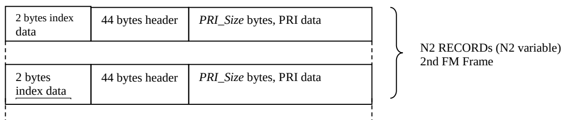
Figure 2.6.5 - 2: Scheme of the Flash Memory frame structure.
