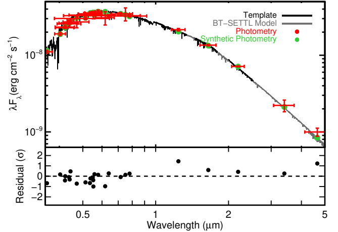
Figure 4. Best-fit spectral template and Goodman spectrum (black) compared to the photometry of HD 63433. Grey regions are BT-SETTL models, used to fill in gaps or regions of high telluric contamination. Literature photometry is shown in red, with horizontal errors corresponding to the filter width and vertical errors to the measurement errors. Corresponding synthetic photometry is shown as green points. The bottom panel shows the residuals in terms of standard deviations from the fit.
