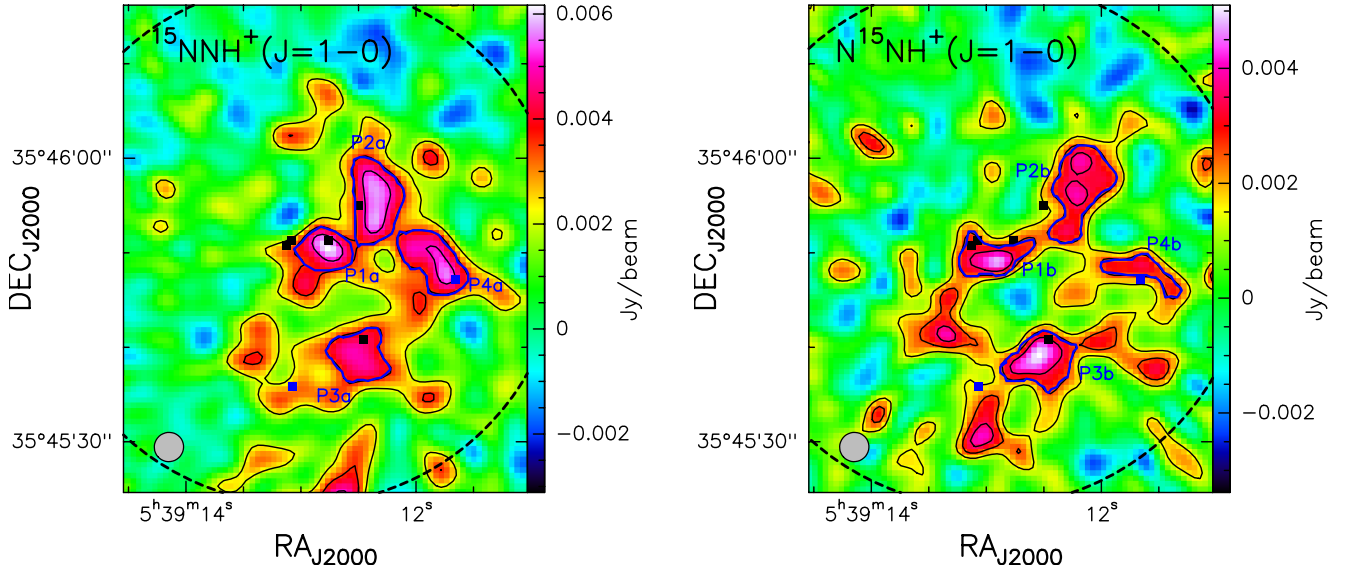
Figure 3. Left panel: Averaged map of ^{15}\text{NNH}^+(1-0) at 90.26 GHz (velocity range between -19.3 and -14.2 \text{ km s}^{-1} ) obtained from the Narrow correlator. The black contour levels are 3, 5 and 7 times the 1\sigma rms of the map, equal to \sim 0.5 \text{ mJy/beam km s}^{-1} . Right panel: Averaged map of the J=1-0 , F=2-1 transition of \text{N}^{15}\text{NH}^+ (main hyperfine component) at 91.20 GHz (velocity range between -19.5 and -15 \text{ km s}^{-1} ) obtained from the Narrow correlator. The black contour levels are 3, 5 and 7 times the 1\sigma rms of the map, equal to \sim 0.72 \text{ mJy/beam km s}^{-1} . In both panels, the blue contours correspond to the 5\sigma level of the averaged maps, from which the spectra have been extracted: P1a, P2a, P3a and P4a from ^{15}\text{NNH}^+ and P1b, P2b, P3b and P4b from \text{N}^{15}\text{NH}^+ . The black and blue squares indicate the positions of the continuum sources and the \text{N}_2\text{H}^+ peak positions (A and B), respectively, as in Fig. 2. The dashed circle represents the NOEMA field of view and the synthesized beam is the ellipse indicated in the lower left corner.
