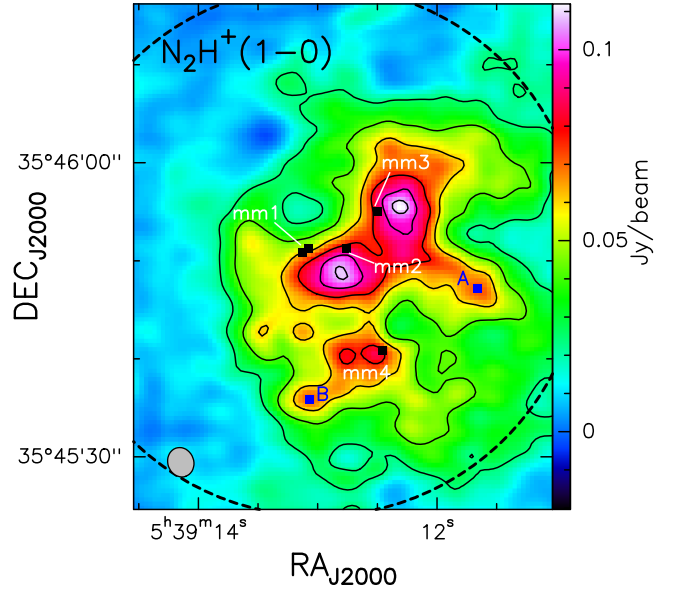
Figure 2. Averaged map of \text{N}_2\text{H}^+(1-0) at 93.1734 GHz (velocity range between -34.6 and -0.1 km s ^{-1} ) obtained from the Widex correlator. The contour levels are 4, 7, 10, 13, 16 and 18 times the 1\sigma rms of the map, equal to \sim 6 mJy/beam km s ^{-1} . The black squares indicate the position of mm1a, mm1b, mm2, mm3 and mm4 as given in the text and in Table 1. The blue squares correspond to the \text{N}_2\text{H}^+(1-0) emission peaks, A and B, described in the text. The dashed circle represents the NOEMA field of view and the synthesized beam is the ellipse indicated in the lower left corner.
