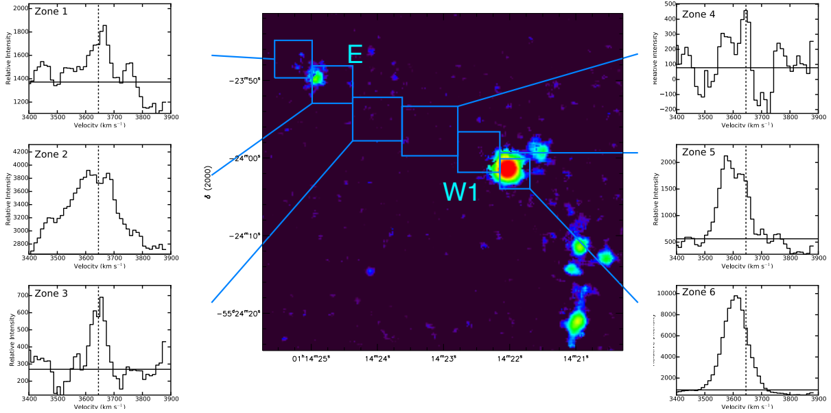
Figure 5. Emission profiles in the region NGC 454 E and NGC 454 W1. The vertical dotted line indicates the systemic velocity adopted V_{hel}=3645 \text{ km s}^{-1} . The horizontal line indicates the mean continuum level. The map corresponds to the monochromatic emission.
