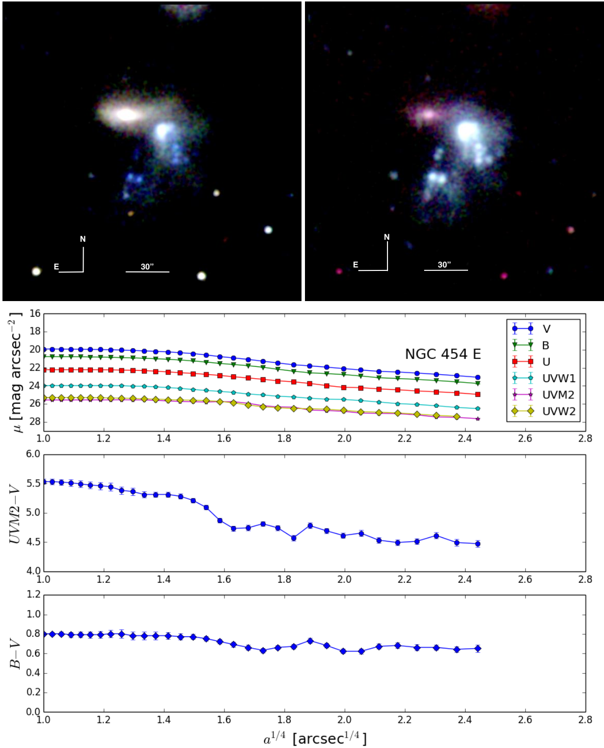
Figure 2. (top panels) Optical image ( U blue, B green, V red), on the left and UV color composite image ( UVW2 blue, UVM2 green, UVW1 red), on the right, of the NGC 454 system as observed by Swift -UVOT. The images have been smoothed 2 \times 2 pixels (resulting 1'' \times 1'' resolution). The total Field of View is 4' \times 4' . (middle panel) Luminosity profiles of NGC 454 E in the optical and NUV bands. Profiles are not corrected for coincidence loss and galactic absorption. (bottom panels) ( M2 - V ) and ( B - V ) color profiles in [AB] magnitudes corrected for galactic absorption.
