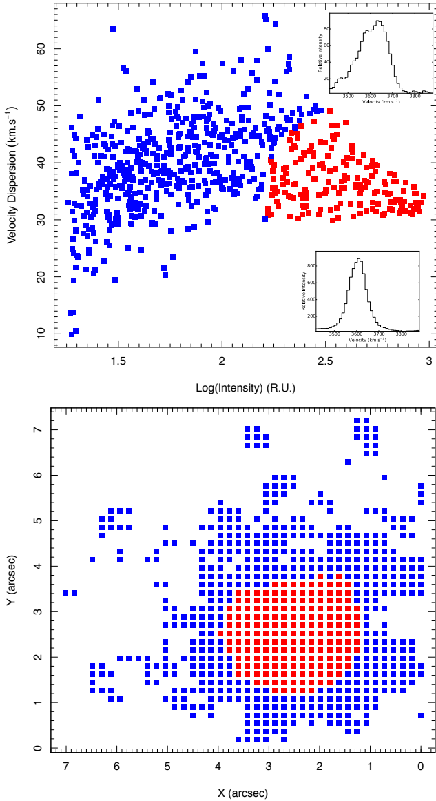
Figure 8. (bottom panel) The 3×3 pixels sampling of the NGC 454 W1 complex. (top panel) (I - \sigma) plot. The colors highlight two regions, the central and outskirts, with different regimes (see Section 5.2 for details). Top profile shows a typical monochromatic emission representative of the blue points, and bottom profile representative of the red points.
