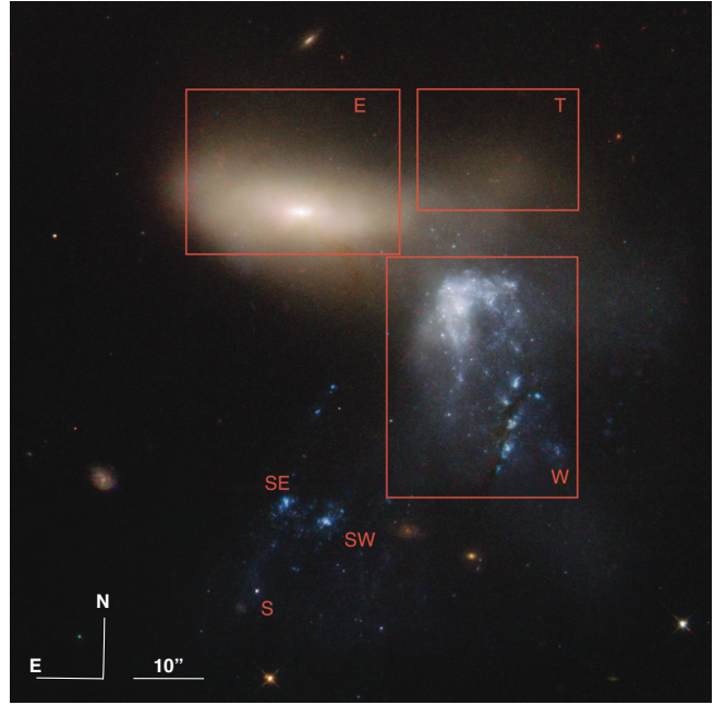
Figure 1. Color composite image of the NGC 454 system obtained with HST-Wide Field Planetary Camera 2 in the F450W (B), F606W (V), and F814W (I) filter by Stiavelli et al. (1998) . The figure highlights the different regions of the system following Johansson (1988) E and W areas include the early-type and the late-type member of the pair, respectively; S, SW and SE are knots likely connected to the W member. T is an area introduced by Stiavelli et al. (1998) (see text). The size of the FOV is 1.66' .
