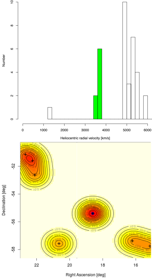
Figure A1. (top panel) Histogram of the heliocentric radial velocity of galaxies within a box of 4 \times 4 \text{ Mpc}^2 in the range 1000 - 6000 \text{ km s}^{-1} . (bottom panel) Spatial distribution of galaxies in green in the top panel, i.e. the neighbors of the NGC 454 system. The map is normalized to the total density. Galaxies in the area are listed in Table A1.
