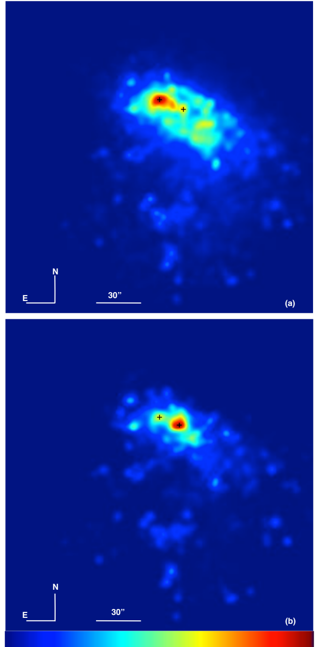
Figure 12. V-band (a) and UV (M2-band, (b)) xz projection of our simulation at the best-fit age; maps are normalized to the total flux within the box, and account for dust attenuation with the same recipes used to provide the SED in Figure 11. The scale is as in Figure 2, with the density contrast being equal to 100. Crosses emphasise the nuclei of the merging galaxies, corresponding to E and Irr in Figure 2 and N-E directions are given to guide the comparison.
