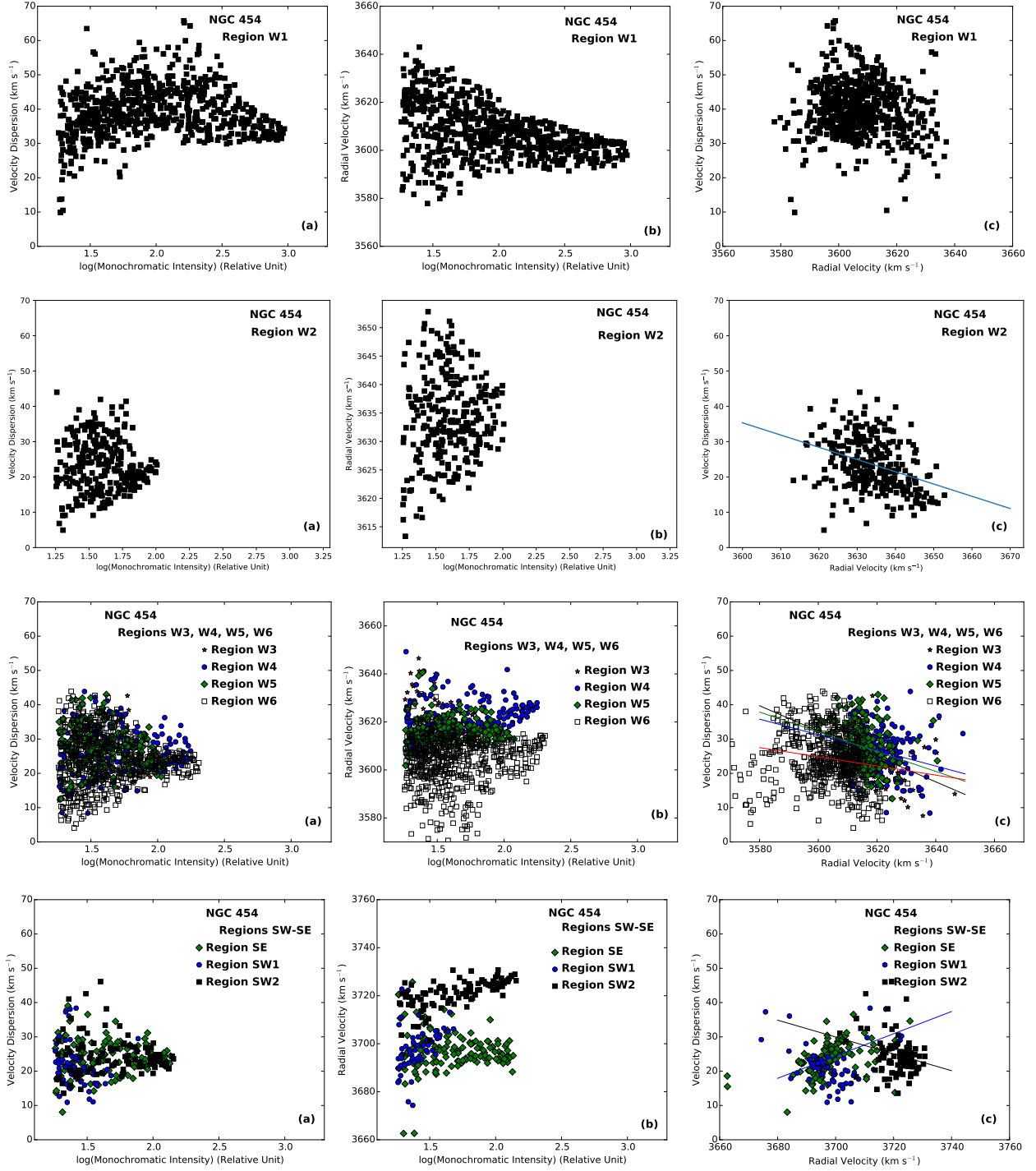
Figure 7. From top to bottom: panels plot (a) (I - \sigma) , panels (b) (I - V_r) , panels (c) (V_{hel} - \sigma) diagnostic diagrams in W1-W6 complexes in NGC 454 W and in the NGC 454 SE and SW complexes. The plot results from a single Gaussian fit to the line profile. Solid lines in V_r - \sigma diagrams represent the linear regressions applied when the Pearson's correlation test is robust.
