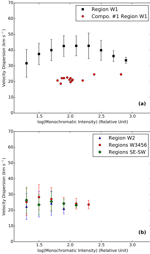
Figure 10. (I - \sigma) diagnostic diagram for the W1 complex (top panel) and for the other complexes in NGC 454 W (bottom panel). The \sigma values are averaged over intensity bins. Red dots on W1 complex show the main component in line profile decomposition shown in Figure 9.
