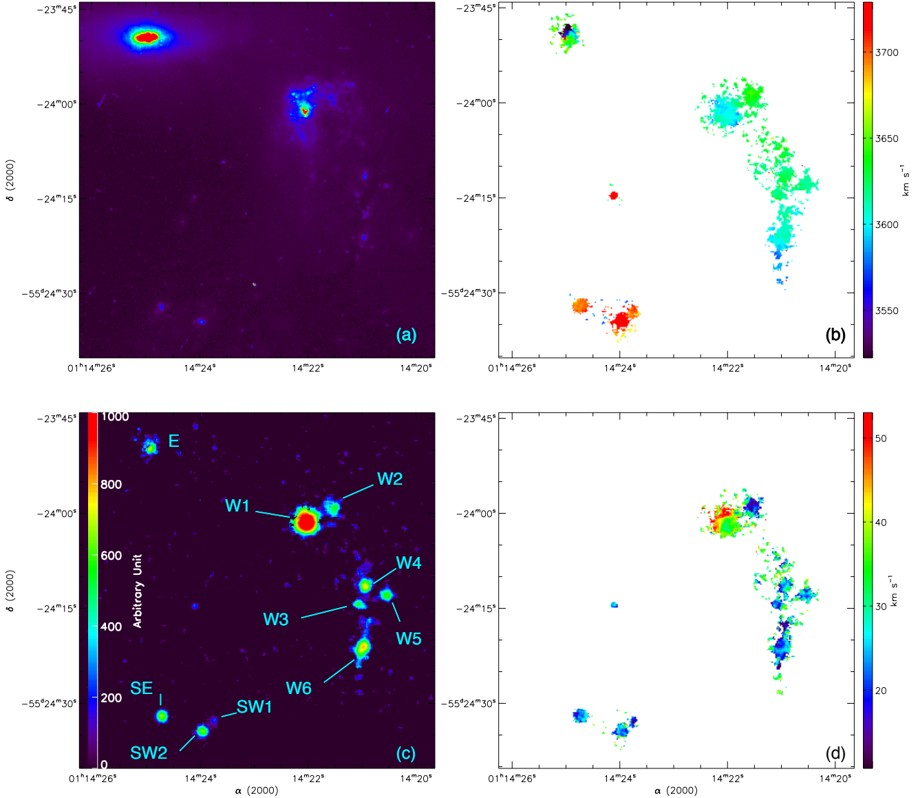
Figure 4. (a) HST F450W image of the NGC 454 system (Stiavelli et al. 1998), (b) 2D velocity field of H \alpha emission, centred on the NGC 454 systemic velocity, (c) monochromatic H \alpha map, and (d) H \alpha velocity dispersion map, corrected from broadening.
