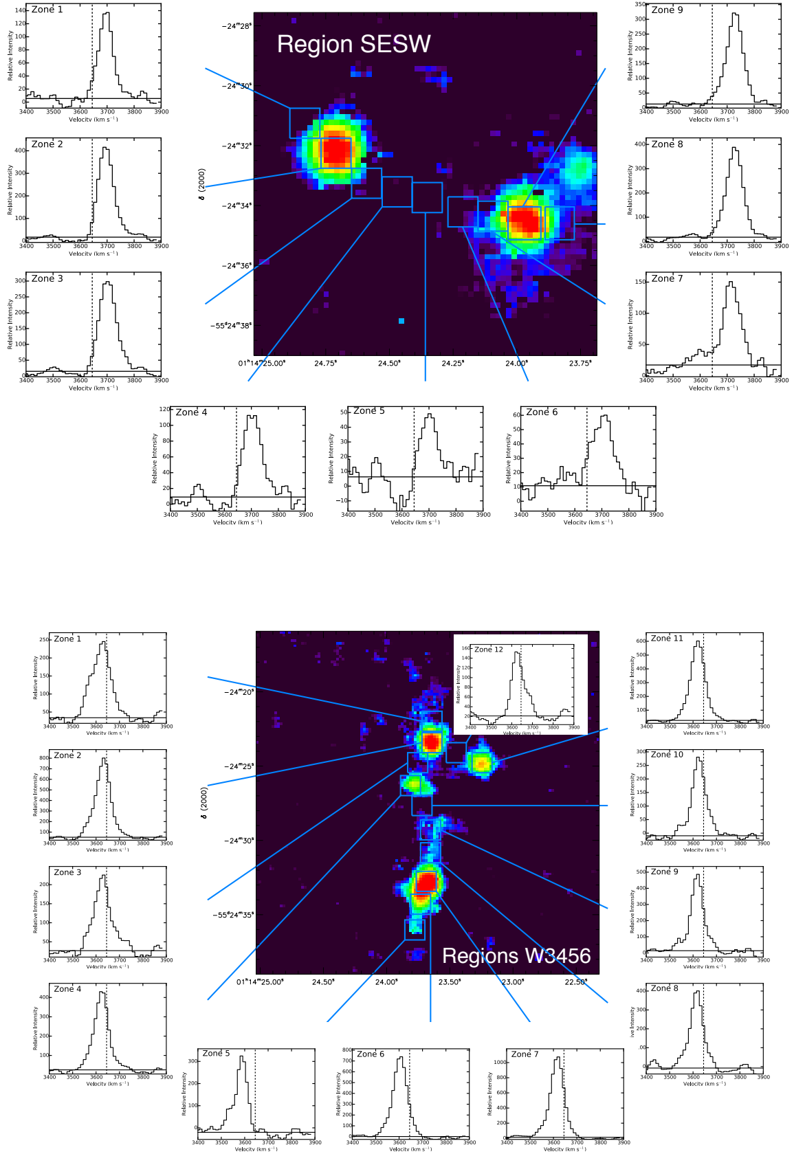
Figure 6. Emission profiles in NGC 454 SE and NGC 454 SW (top panel) and in the NGC 454 W region between W3 and W6 complexes (bottom panel). The vertical dotted line indicates the systemic velocity adopted V_{hel}=3645 \text{ km s}^{-1} . The horizontal line indicates the mean continuum level. The map corresponds to the monochromatic emission.
