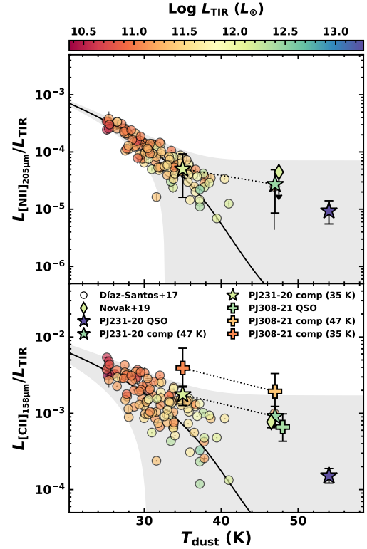
Fig. 6. [\text{NII}]_{205\mu\text{m}} and [\text{CII}]_{158\mu\text{m}} line deficits (top and bottom panel, respectively) with respect to the total IR luminosity ( L_{\text{TIR}}(8-1000\mu\text{m}) ) for quasars PJ231–20 and PJ308–21 and the companion galaxies and the LIRG sample of Díaz-Santos et al. (2017) as a function of dust temperature and color-coded by \log L_{\text{TIR}} . We also report the measurements obtained for the z = 7.54 quasar ULAS J1342+0928 (Novak et al. 2019). The sources in system PJ231–20 are indicated by stars, and those in system PJ308–21 are marked with crosses. For the companion galaxies we report the cases with assumed dust temperatures of 47 K and 35 K. These points are connected by a dashed line. The solid lines are the best fit to the LIRG sample performed in Díaz-Santos et al. (2017) using the model L_{\text{line}}/L_{\text{FIR}} = \epsilon_0 \exp(-S_{63}/S_{158})/\delta with (\epsilon_0, \delta) = ((1.26 \pm 0.16) \times 10^{-3}, 0.50 \pm 0.04) for the [\text{NII}]_{205\mu\text{m}} line, and (\epsilon_0, \delta) = ((14.0 \pm 0.9) \times 10^{-3}, 0.68 \pm 0.04) for [\text{CII}]_{158\mu\text{m}} line. We scaled the best fits by a constant factor because different FIR luminosity definitions were employed by Díaz-Santos et al. (2017). The best-fit scaling values are 0.56 for [\text{NII}]_{205\mu\text{m}} line and 0.44 for [\text{CII}]_{158\mu\text{m}} line. The gray shaded area represents the 1\sigma scatter of the relation. The Novak et al. (2019) points were slightly shifted along the dust temperature axis (assumed to be 47 K) for a better visualization of the data.
