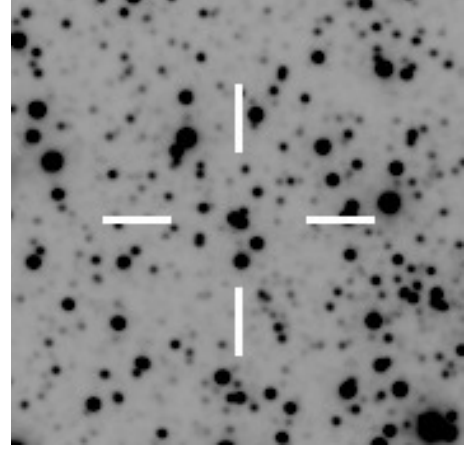
Fig. 4. Image of star 2461 in the VVV survey, indicating a blend of stars. Extraction of \sim 20 arcsec. North is 45^\circ anticlockwise.
