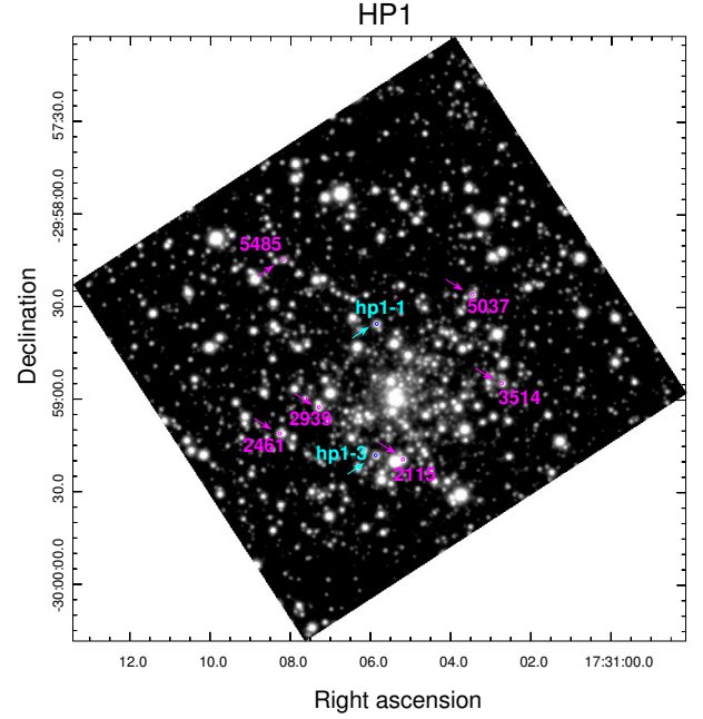
Fig. 2. z image from the VVV survey, indicating the location of the sample stars.
