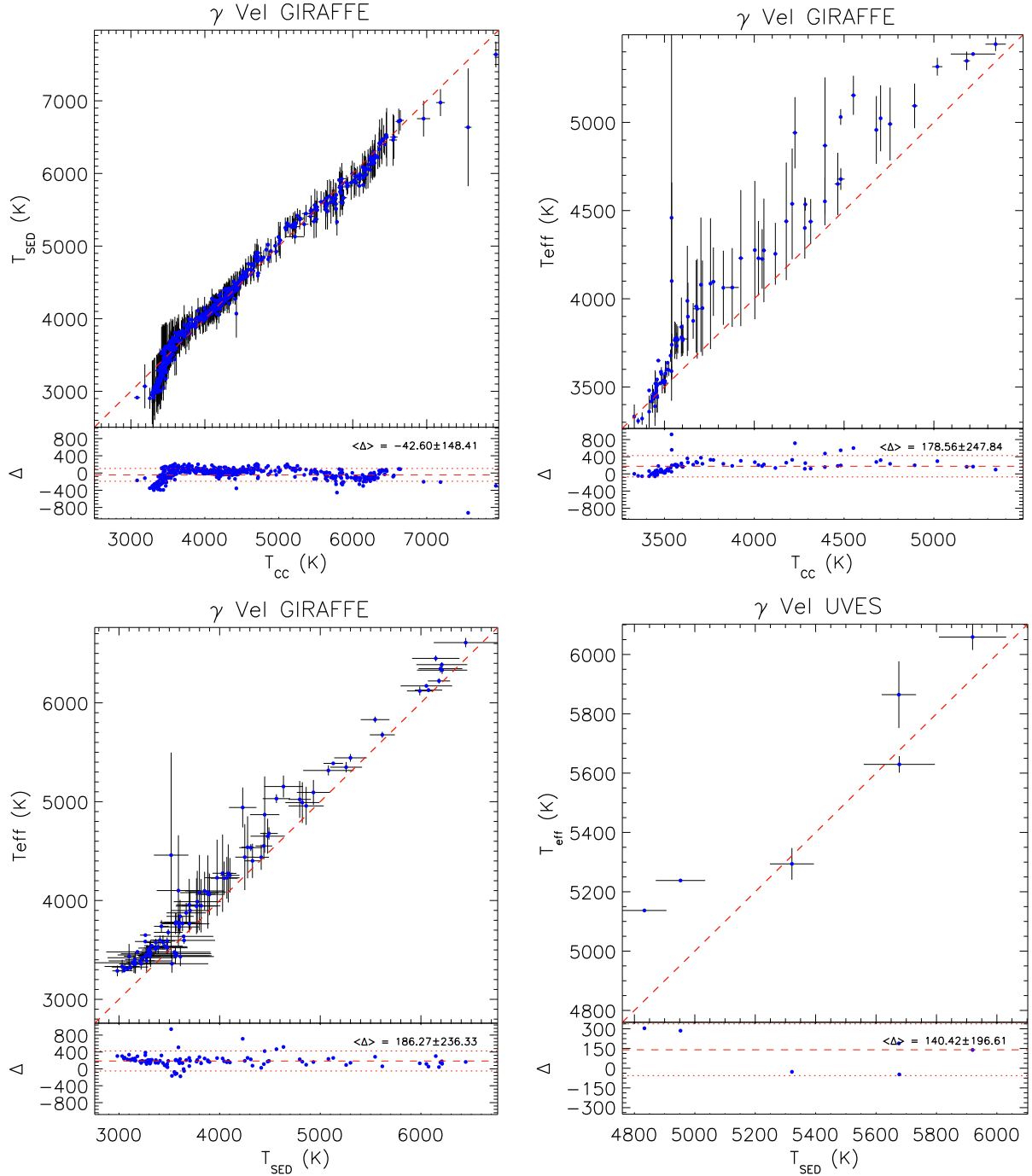
Fig. C.2. Top left panel: comparison of T_{\text{SED}} and T_{\text{CC}} for all GIRAFFE spectra in the \gamma Vel field for which \chi^2_{\text{CC}} < 7 , irrespective of Li and RV membership. Top right panel: recommended T_{\text{eff}} vs. T_{\text{CC}} for GIRAFFE spectra of probable members of \gamma Vel. Bottom left panel: recommended T_{\text{eff}} vs. T_{\text{SED}} for GIRAFFE spectra of probable members of \gamma Vel. Bottom right panel: recommended T_{\text{eff}} vs. T_{\text{SED}} for all UVES spectra in the \gamma Vel field.
