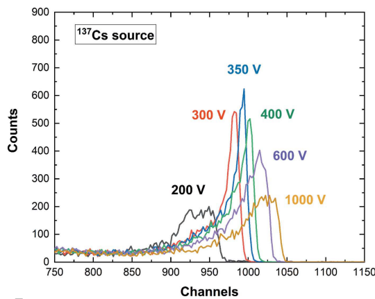
Figure 7 662 keV photopeaks of the measured ^{137}\text{Cs} spectra from a collecting anode strip at different cathode bias voltages; fixed drift strip voltages (adjacent drift strips: -100 V; central drift strips: -200 V) are used. The detector, irradiated in PTF geometry, shows the best energy resolution (1.3% FWHM at 661.7 keV) at a cathode voltage of -350 V ( 583 V \text{cm}^{-1} ).
