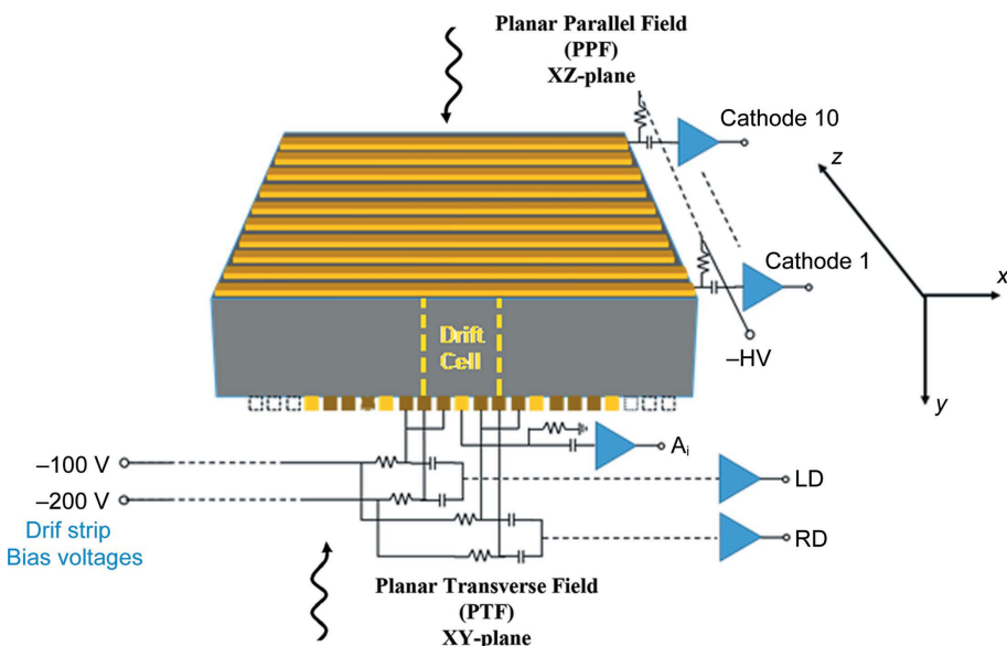
Figure 3 Layout of a single drift cell of the 3D drift strip CZT detectors. Each drift cell ( 1.6 \text{ mm} \times 6 \text{ mm} \times 20 \text{ mm} ) contains a collecting anode strip and four drift strips, two RDs and two LDs of the collecting strip. The bias voltage values are optimized to collect electron charges on the collecting anode. The PTF and PPF irradiation geometries are also shown.
