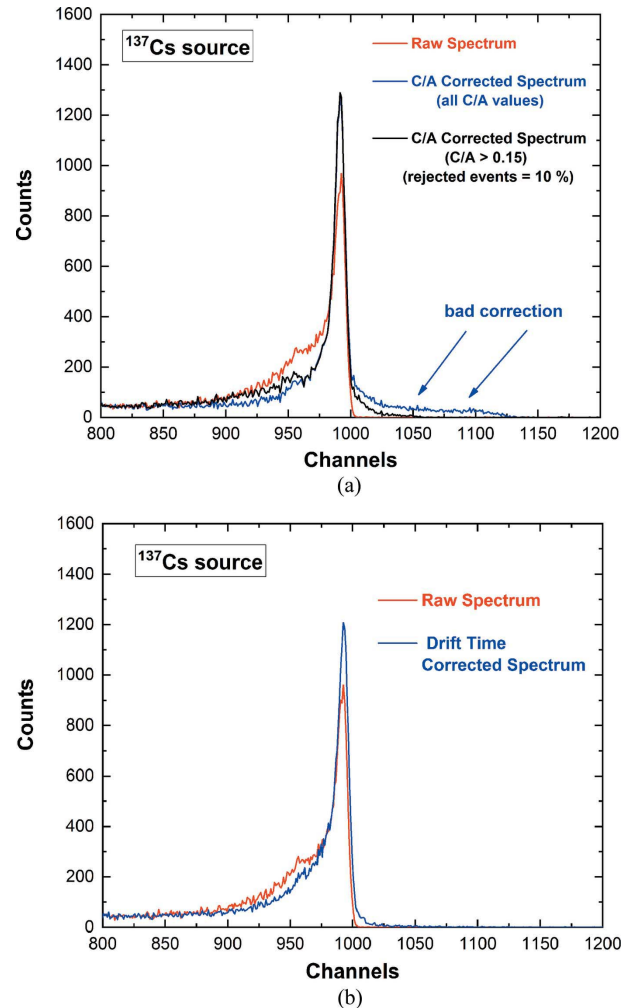
Figure 13 Measured ^{137}\text{Cs} energy spectra corrected with equation (2). (a) C/A ratio correction (black and blue lines). (b) Drift time correction (blue line). Energy resolutions of 1% and 1.16% FWHM at 661.7 keV are obtained for the C/A ratio and drift time correction, respectively.
