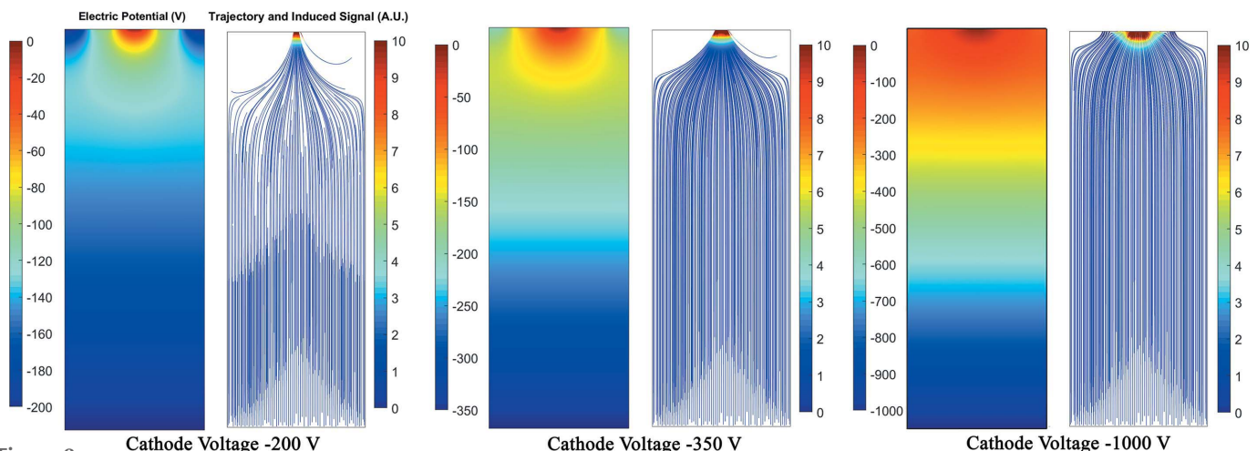
Figure 8 Calculated electric potential and simulated electron induced current at different cathode voltages (adjacent drift strips: -100 V; central drift strips: -200 V). The results clearly show that the induced current on the collecting anode strip is enhanced at -350 V.
