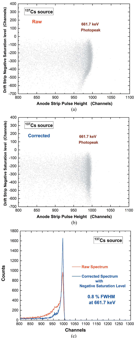
Figure 14 (a) Raw and (b) corrected [equation (2)] scatter plots of the negative saturation level versus the height of pulses from a collecting anode strip. (c) Excellent energy resolution is obtained after correction considering only the induced-charge pulses with negative saturation level.
