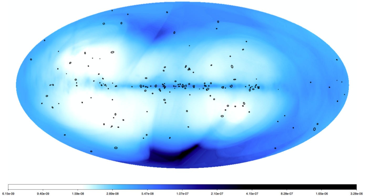
Fig. 7: Sky map of 4\sigma sensitivity in the energy range 100 MeV – 10 GeV in Galactic coordinates and Hammer-Aitoff projection; the hypothesis of a PL spectral model with \alpha = 2.1 , in \text{ph cm}^{-2}\text{s}^{-1} . The 95% elliptical confidence regions of the 2AGL sources are superimposed in black.
