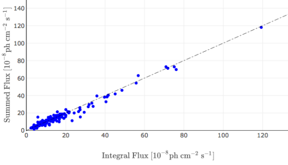
Fig. 6: Comparison of the energy flux in the energy range 100 MeV – 10 GeV estimated from the sum of bands (ordinate) and the fit to the full band (abscissa) for all 2AGL sources, in 10^{-8} \text{ ph cm}^{-2} \text{ s}^{-1} . No obvious bias can be observed.
