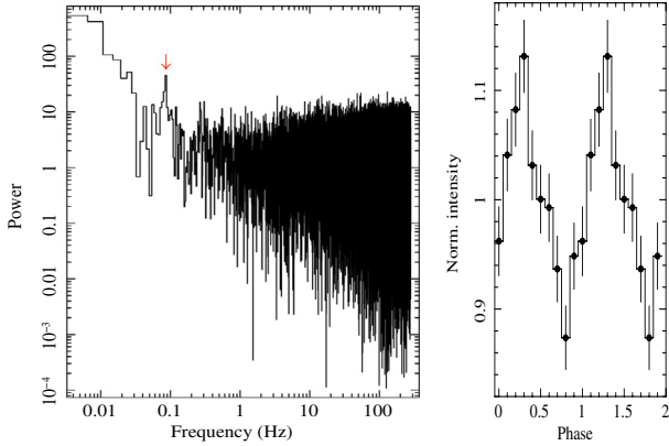
Fig. 4. Left: Fourier power spectrum of the Swift /XRT WT mode data (0.3–10 keV) collected at the beginning of the outburst. The peak corresponding to the 0.086 Hz signal is indicated by the red arrow. Right: Folded profile obtained by folding the WT at the 11.6 s candidate period (see Sect. 3.2 for details).
