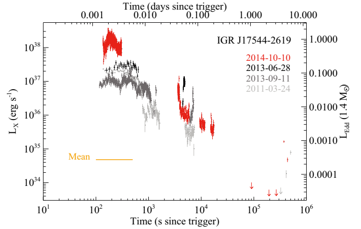
Fig. 3. Bolometric X-ray luminosity light curves of the brightest outbursts recorded by Swift for this source. Red: 2014 October 10, light grey: 2011 March 24, black: 2013 June 28, dark grey: 2013 September 11. The horizontal (orange) line marks the average level for this source.
