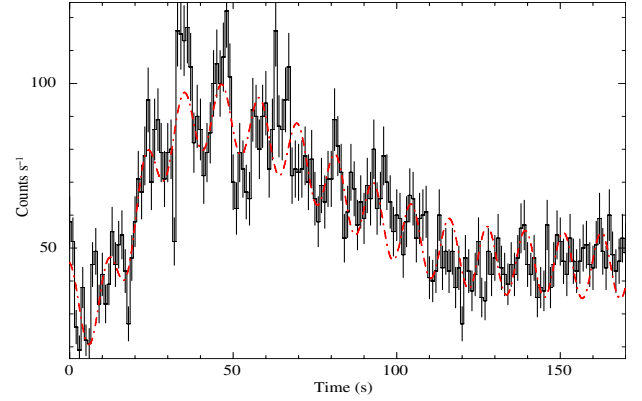
Fig. 5. Swift /XRT WT (0.3–10 keV) light curve (black) fitted with a model consisting of a constant plus two Gaussians for the continuum, and an additional sinusoidal component to account for the modulation.
