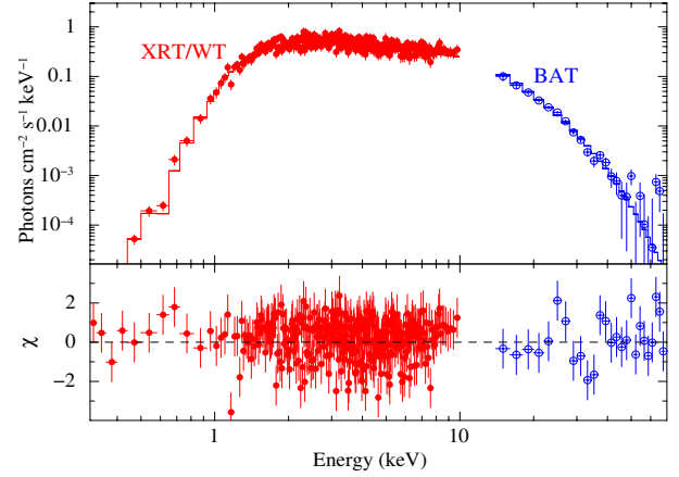
Fig. 2. Spectroscopy of the 2014 October 10 outburst of IGR J17544–2619. Top panel: simultaneous XRT/WT data (filled red circles) and BAT data (empty blue circles) fit with an absorbed power law with a high energy exponential cut-off model. Bottom panel: residuals of the fit (in units of standard deviations).
