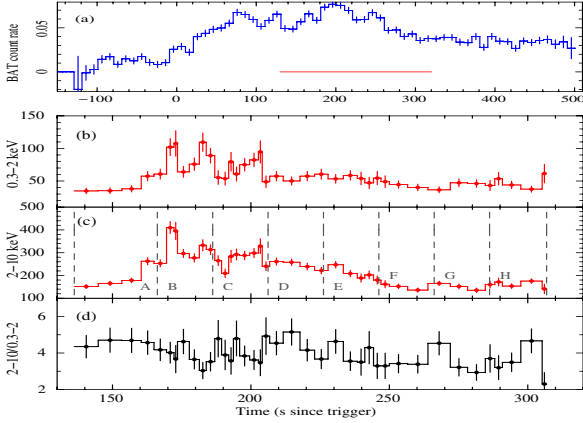
Fig. 1. Light curves of the 2014 October 10 outburst of IGR J17544–2619. a) BAT (14–150 keV, 10 s binning): the red horizontal line marks the XRT data span; b) XRT soft band (0.3–2 keV, at 30 counts bin -1 ); c) XRT hard band (2–10 keV, at 30 counts bin -1 ); d) XRT hardness ratio (2–10 keV/0.3–2 keV). The dashed vertical lines mark the time selections for BAT and XRT spectroscopy (Sect. 3.1).
