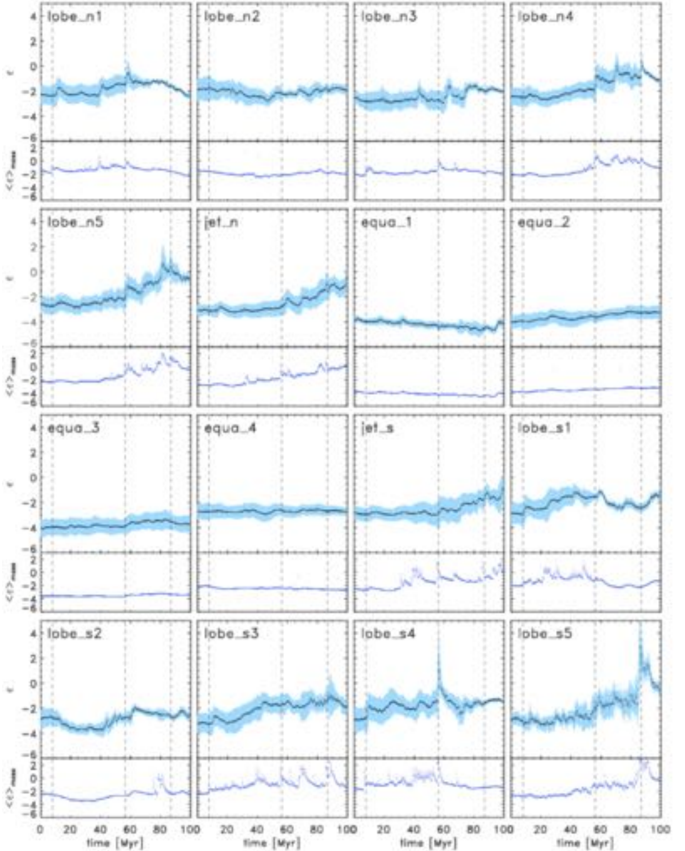
Figure 8. Lagrangian analysis: temporal evolution of enstrophy as recorded by the 16 different tracer families (Fig. 7). Each top/bottom panel show the median/mean of the recorded enstrophy, respectively. The blue bands mark \pm 1 standard deviation. The unit of the y-axis is \log_{10}(\text{Myr}^{-2}) . The three vertical dashed lines highlight the events of strongest enstrophy and AGN power (see Fig. 1).
