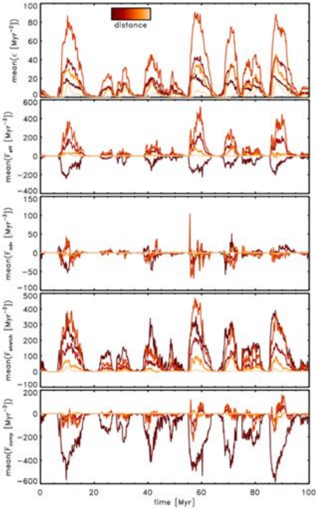
Figure 4. Eulerian analysis: evolution of the mean values of enstrophy (top row), effective dynamical term (second row), advection (third row), stretching (fourth row), and compression term (fifth row). The means are computed within pairs of short cylinders aligned with the bipolar jet path, with a cylindrical radius of 15 kpc and increasing distance from the AGN ( \approx 1, 9, 18, 36, 72 kpc; dark red to bright yellow colour).
