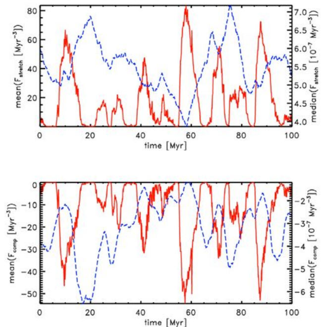
Figure 3. Eulerian analysis: evolution of the mean (red solid) and median (blue dashed) of the stretching (top) and compressive/rarefaction (bottom) terms computed on the grid, including the dominant positive/negative range. (Notice the respective, different left/right y-axis labelling).
