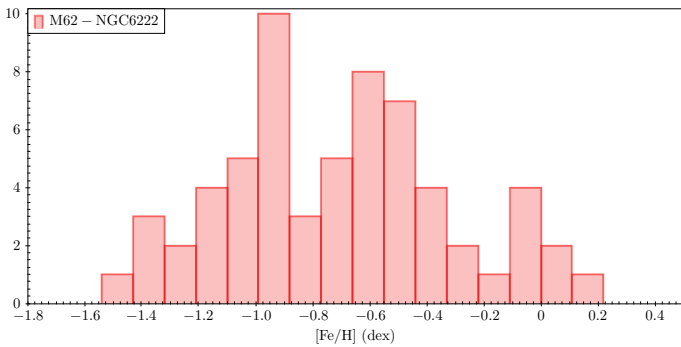
Fig. 22. Same as in Fig. 21, but for RR Lyrae stars in M62.
