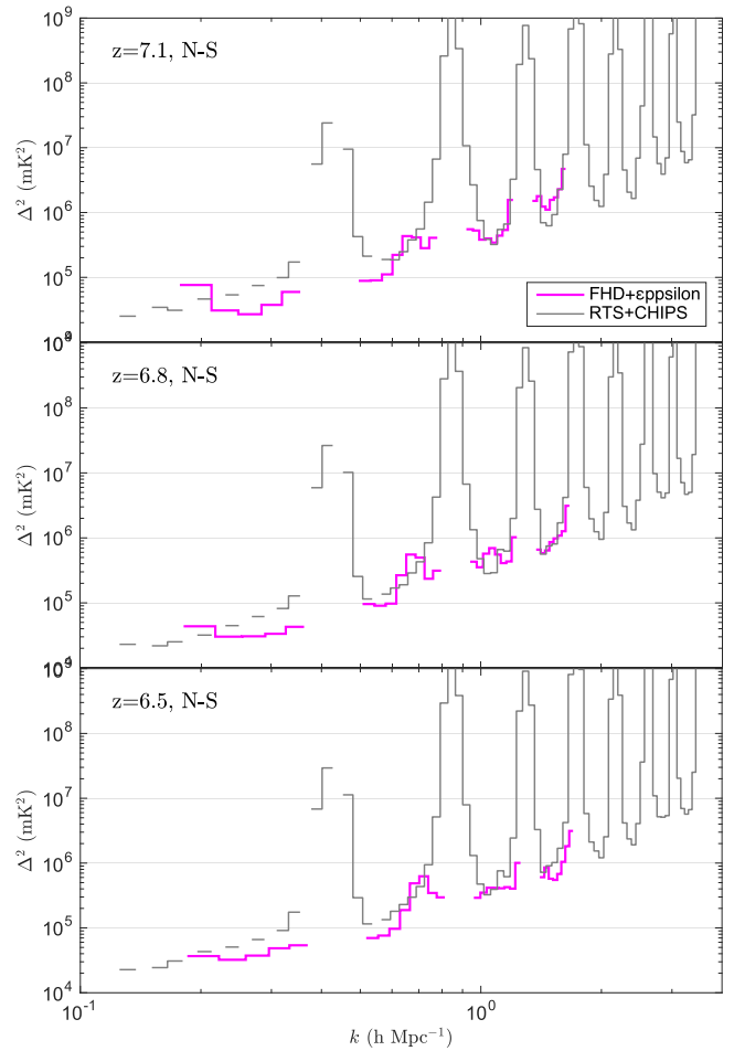
Figure 16. Here we compare the upper limits from the FHD+ \epsilon psilon pipeline with those from the RTS+CHIPS pipeline. The magenta lines are repeated from Figure 15, and the gray lines are the power plus 2\sigma thermal error bars generated by CHIPS. Due to the logarithmic binning used by CHIPS, some bins are empty, resulting in gaps in the spectra. CHIPS does not excise the coarse-band harmonic lines, and so we see their strong effect where there are gaps in the magenta lines. The RTS+CHIPS pipeline accesses larger k modes because the data is processed at 80 kHz, whereas the FHD+ \epsilon psilon pipeline averages to 160 kHz when gridding. The most notable differences are the ability of the RTS+CHIPS pipe to access lower k modes, while the FHD+ \epsilon psilon pipe suppresses more power before and after the first coarse-band harmonic. While the different analysis methods result in slightly different upper limits, they are generally in agreement.
