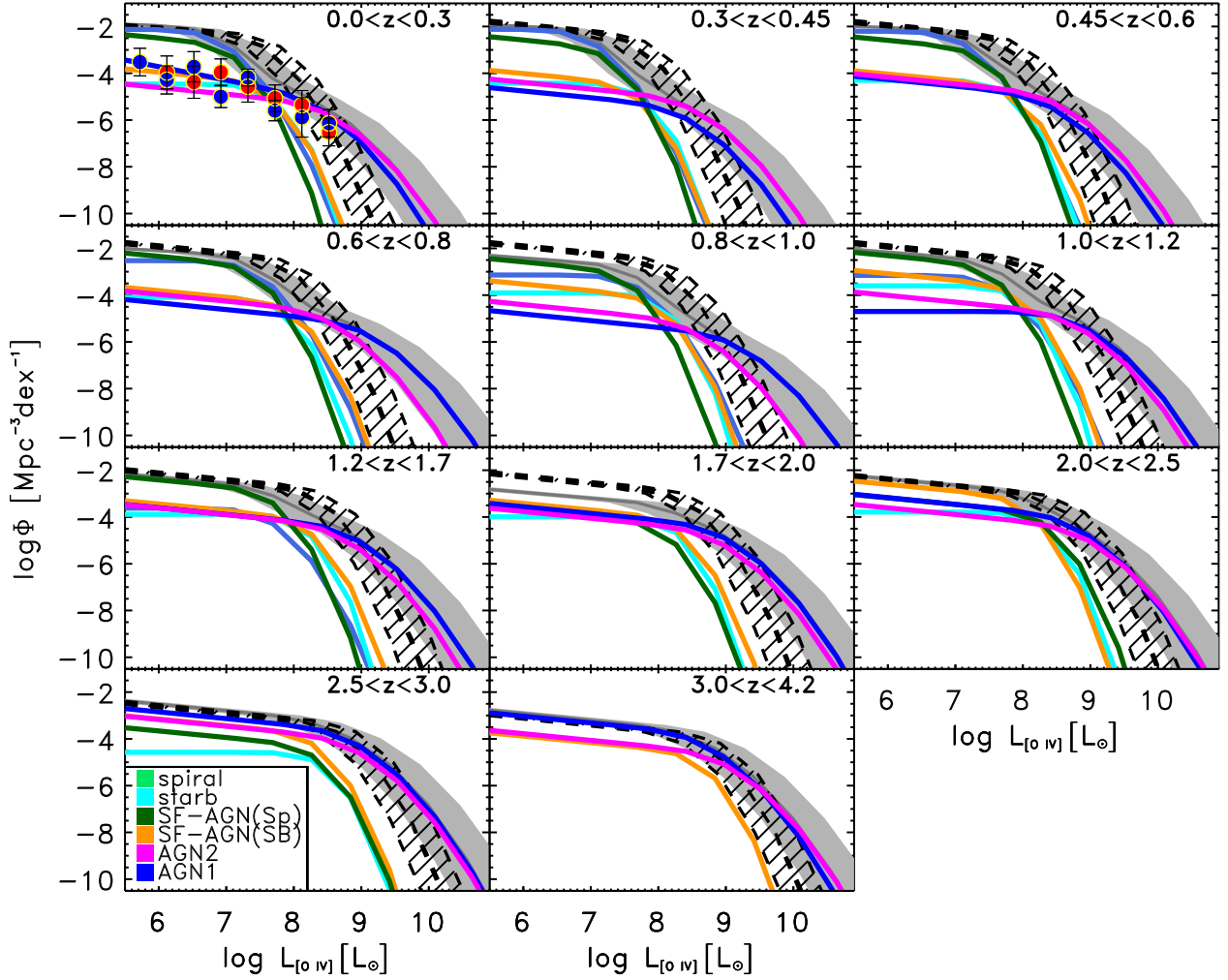
Figure 12. LF of the [O IV] 25.9 \mu\text{m} line in different redshift intervals, obtained by converting the total IR LF of Gruppioni et al. (2013) through the L_{\text{line}}-L_{\text{IR}} relations found in Section 6. The different coloured lines represent the different IR populations (evolved and converted separately, according to their average AGN fraction), whose sum is shown by the grey band. The black dashed line shows the LF obtained by converting the total IR LF using the average L_{[\text{O IV}]}-L_{\text{IR}} relation. The filled symbols in the 0.0 < z < 0.3 panel show the [O IV] LF derived by Tommasin et al. (2010) for Seyfert 1 (red circles) and Seyfert 2 (blue circles) galaxies.
