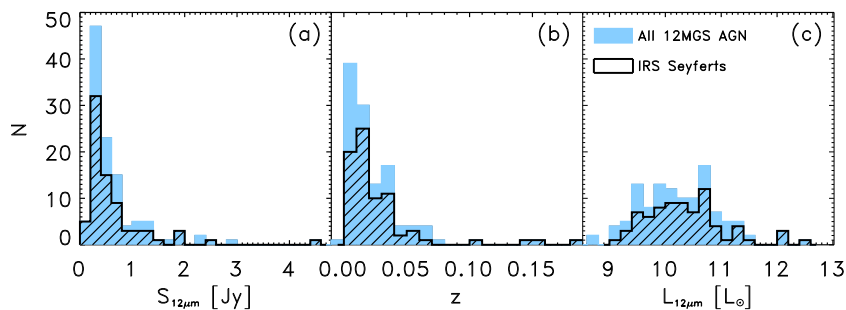
Figure 1. Distribution of (a) 12-μm flux, (b) redshift and (c) 12-μm luminosity of the 76 Seyferts with Spitzer -IRS low-resolution spectra (black hatched histogram) versus entire 12MGS sample of optically classified AGN (blue filled histogram).
