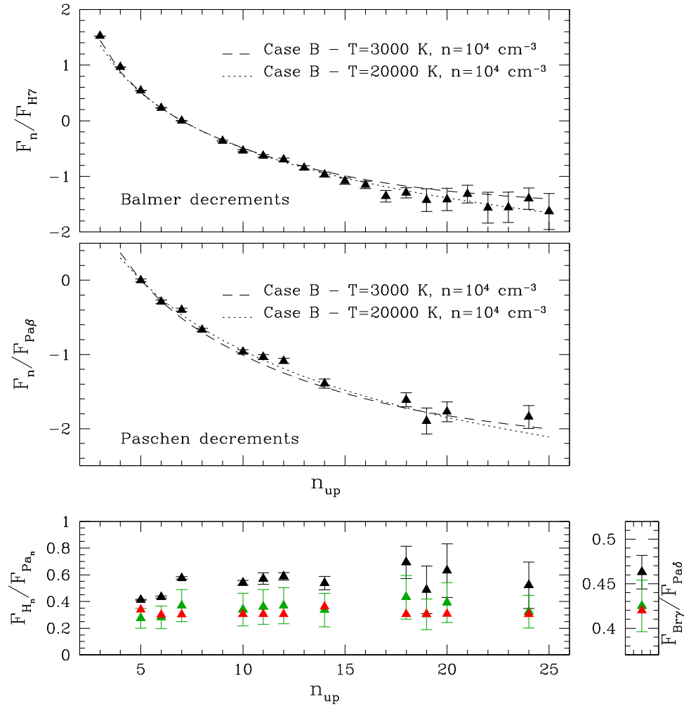
Figure 2. Top and middle panels: Balmer and Paschen observed decrements fitted with case B recombination models. The best fits correspond to n = 10^4 \text{ cm}^{-3} and 3000 \leq T \leq 20,000 \text{ K} , obtained by normalizing the Paschen decrements to the P\beta and the Balmer decrements to the H7 . In both panels, we plot only the lines that are not blended with lines from other species and not contaminated by artifacts or sky line residuals in the spectral images. Bottom panel (left): ratios of Balmer and Paschen lines coming from the same upper level. Black symbols are the observed ratios, red symbols are the theoretical values, and green symbols are the observed ratios once dereddened for A_V = 0.2\text{--}0.4 \text{ mag} (estimated for R_V = 3 ). Bottom panel (right): same as in the left panel for the \text{Br}\gamma/\text{Pa}\delta ratio.
