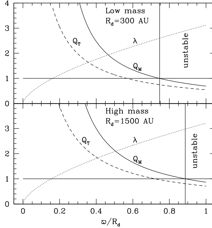
Fig. 1.4 Radial profiles of the Toomre stability parameter Q_T , the magnetic stability parameter Q_M , and the local mass-to-flux ratio \lambda in typical disks around high-mass stars (lower panel) and low-mass stars (upper panel). These profiles are obtained from the disk models of Shu et al. (2007) with an aspect ratio \propto \varpi^{1/4} . The radial coordinate is normalized to the disk radius R_d .
