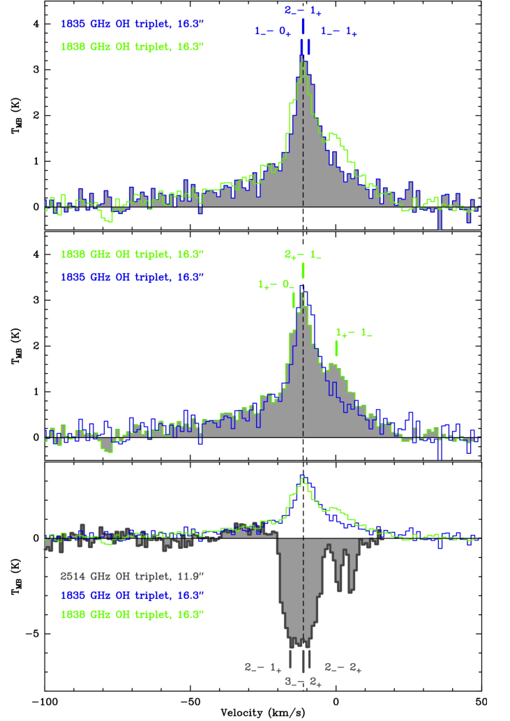
Fig. 2. Top panel: 1835 GHz OH triplet (blue line and grey histogram), overlaid with the 1838 GHz triplet (green line). Middle panel: The 1838 GHz OH triplet (green line and grey histogram), overlaid with the 1835 GHz triplet (blue line). Bottom panel: The 2514 GHz OH triplet (dark grey and grey histograms), overlaid with the 1838 GHz (green line) and 1835 GHz (blue line) triplets. In all panels, the lines were observed at the Cep A HW2 position, indicated in Figure 1, and the three components of the triplets are indicated in the same colour as the considered triplet: see Tables 1 and 2. The vertical dashed line is at the v_{\text{lsr}} of the cloud ( -11.2\ \text{km s}^{-1} ; e.g. Narayanan & Walker 1996; Gómez et al. 1999). In the top and middle panels, the spatial and spectral resolutions are 16''.3 and 1.25\ \text{km s}^{-1} , respectively. In the bottom panel, they are 11''.9 and 0.91\ \text{km s}^{-1} .
