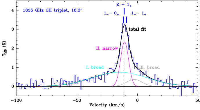
Fig. A.1. Triple-Gaussian fit of the 1835 GHz OH triplet (blue line, from Figure 2): blueshifted (light blue line), ambient (pink line), redshifted (grey line) components, and total fit (black line). The vertical dashed line is at the cloud v_{\text{lsr}} of -11.2 \text{ km s}^{-1} (Narayanan & Walker, 1996; Gómez et al., 1999).
