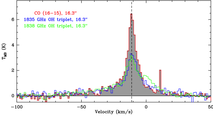
Fig. 3. CO (16–15) transition (red line and grey histograms) at the Cep A HW2 position, overlaid with the 1835 GHz and 1838 GHz triplets (blue and green lines, from Figure 2). The spatial and spectral resolutions of the CO line are 16''.3 and 1.24 km s ^{-1} . The vertical dashed line is at the cloud v_{\text{lsr}} of -11.2 km s ^{-1} (Narayanan & Walker, 1996; Gómez et al., 1999).
