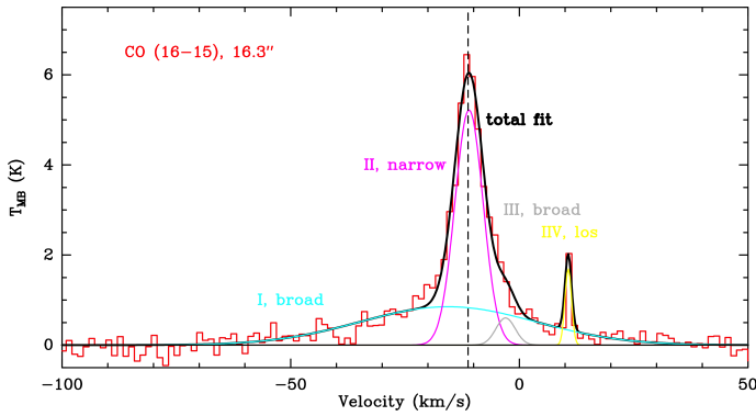
Fig. A.2. Triple-Gaussian fit of the CO (16–15) transition (red line, from Figure 2): blueshifted (light blue line), ambient (pink line), redshifted (grey line) components, and total fit (black line). An additional component has been fitted with respect to the OH line in Figure A.1: a narrow CO feature at 10.7 \text{ km/s} due to mesospheric CO over-compensated by the correction for the atmospheric opacity and well reproduced by a fourth Gaussian (yellow line). The vertical dashed line is at the cloud v_{\text{lsr}} of -11.2 \text{ km s}^{-1} (Narayanan & Walker, 1996; Gómez et al., 1999).
