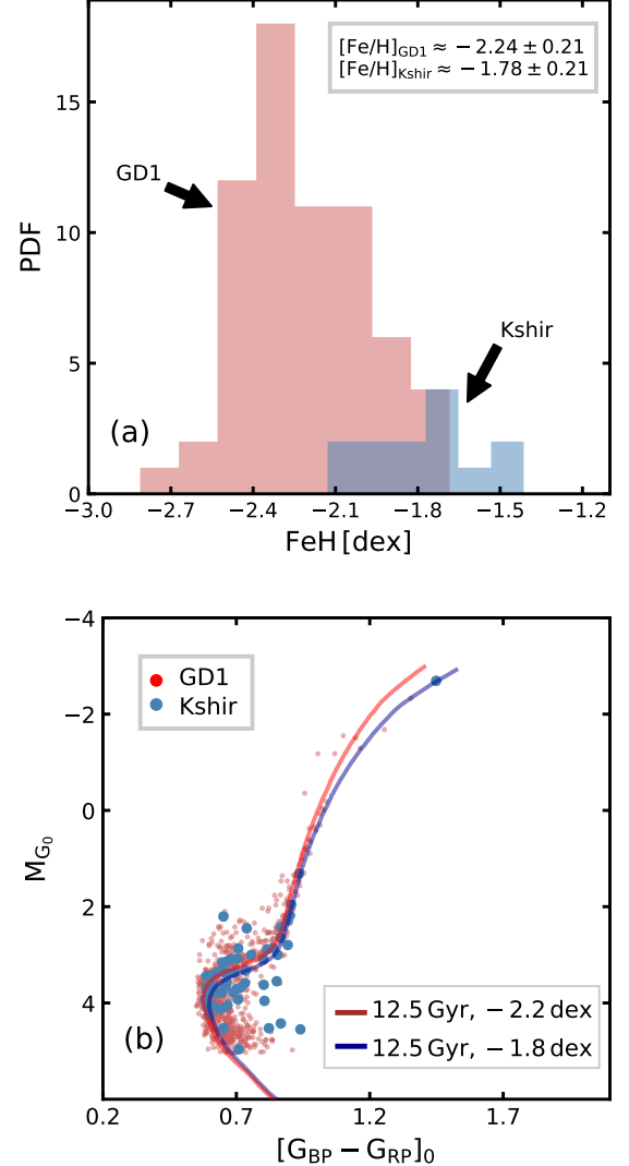
FIG. 2.— Metallicity and photometry of GD-1 and Kshir. Top panel: [\text{Fe}/\text{H}] distribution of spectroscopically-confirmed members of GD-1 (red) and Kshir (blue) stars. Bottom panel: Gaia (de-reddened) color-magnitude diagram of all member stars of Kshir and GD-1, previously shown in Fig 1. The absolute magnitude were then obtained by correcting the observed magnitude value for the orbital distance of each star. Two SSP template models, corresponding to the mean metallicity values of the streams, are also shown.
