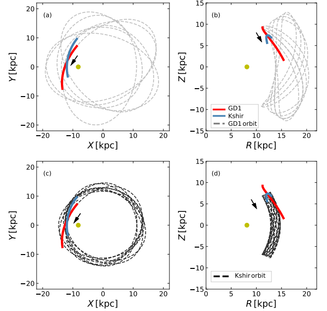
FIG. 3.— The orbital trajectories of GD-1 and Kshir in the Galactocentric Cartesian system. Top panels: GD-1’s orbit (silver). For perspective, the current locations of GD-1 (red) and Kshir (blue) are also shown. The Galactic centre lies at the origin and the Sun (yellow dot) is at (X,Y,Z) = (-8.122, 0, 0) \text{ kpc} . The orbit was integrated backwards in time for 3 Gyr. The arrows represent the direction of motion of the structures. Bottom panels: As above, but showing Kshir’s orbit (black).
