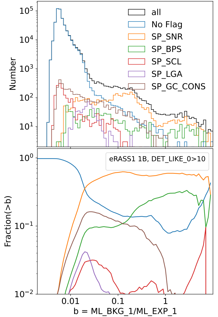
Fig. 7. Top panel: distribution of local background rate level ( \text{ML\_BKG\_1}/\text{ML\_EXP\_1} , in units of \text{counts arcmin}^{-2} \text{ s}^{-1} ) for sources with and without flags and \text{DET\_LIKE\_0} > 10 . Bottom panel: the fraction of each corresponding sub-sample among all the sources above any background level.
