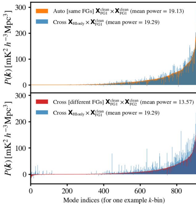
Figure 12. Amplitude of all Fourier modes P(k) \propto \text{Re} \{ \tilde{X}_A(k) \cdot \tilde{X}_B^*(k) \} in the range 0.0590 < k < 0.0687 \text{ h Mpc}^{-1} , which corresponds to one chosen k -bin in the spherically averaged power spectrum. The average of these modes, stated in the legend for each scenario, will represent the spherically averaged power spectrum value for the particular k -bin. The top panel shows the equivalence in signal-loss between autocorrelation and cross-correlation. The lower panel shows how signal loss can be larger where a different set of modes has been projected out in the foreground clean shown by the red results which is the cross-correlation between two different simulated foreground regions.
