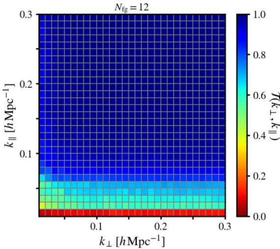
Figure 6. Similar to Fig. 5, this shows the foreground transfer function but now in cylindrical k_{\perp}, k_{\parallel} space where N_{\text{fg}} = 12 PCA modes have been removed. This is for the noise-free case.
