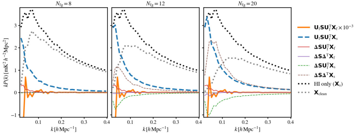
Figure 3. Contributions to signal loss from the decomposed terms in equation (9). Each power spectra shows the cross-correlation between the original-HI and a subtracted term in the foreground clean. The different panels represent different numbers of PCA modes removed ( N_{fg} ). The solid lines indicate residual foreground contributions, whereas the dashed lines indicate H I signal contributions. The thin lines indicate perturbed contributions from \Delta caused by the presence of signal in the eigenmode estimation. For reference, we also include the pure H I-power (black dotted) along with the total cleaned result X_{clean} (grey dotted).
