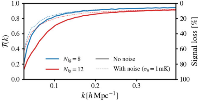
Figure 5. Foreground transfer functions \mathcal{T}(k) constructed using equations (11) and (10) for the MD1GPC simulations for different numbers of PCA modes removed (given by N_{\text{fg}} ). The solid lines indicate noise-free simulations; the thin dashed lines are for cases where white noise with rms \sigma_n = 1 mK, which dominates over the H\text{I} , is added to the simulated observations.
