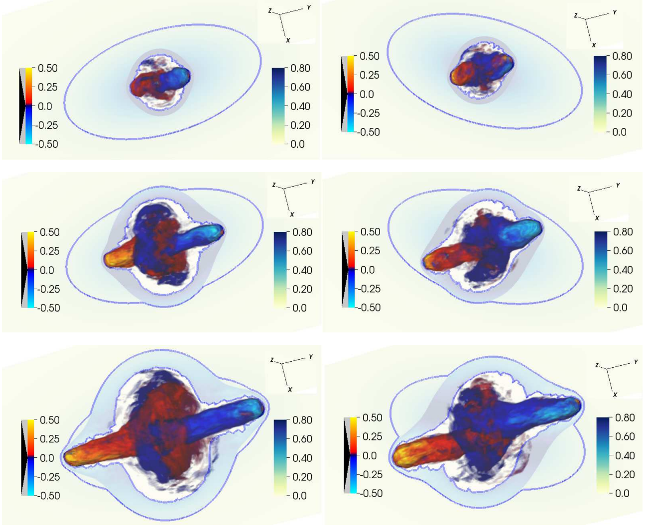
Fig. 7. Evolution of cases E and F. The three panels on the left are for case E at times respectively 9.6 \times 10^5 yrs, 1.8 \times 10^6 yrs, and 2.6 \times 10^6 yrs, from top to bottom, while the three panels on the right are for case F at times respectively 9.6 \times 10^5 yrs, 1.6 \times 10^6 yrs, and 2.3 \times 10^6 yrs, from top to bottom. The distribution of y velocity component is represented by a volume rendering, with blue colors representing negative values and red-yellow colors representing positive values. Superimposed, we also show a cut of the density distribution in the x - y plane, while the blue lines are density iso-contours at \rho = 0.2\text{cm}^{-3} on the same plane.
