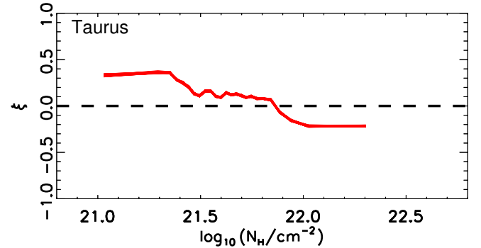
Fig. B.2. Histogram shape parameter, \xi , as a function of \log_{10}(N_H/\text{cm}^{-2}) in the Taurus region. The values are obtained using the \tau_{353} map at 10' resolution and maps of the Stokes parameters Q_r and U_r that correspond to 1000 random-noise realizations. Each realization is generated using a Gaussian probability density function centred on the measured values Q and U with variances \sigma_Q^2 and \sigma_U^2 . By joining the values at each N_H bin, we find a trend very close to the black line in Fig. 7, with little dispersion from the noise; much larger are the uncertainties in evaluating \xi at each N_H bin, as given in Fig. 7 but not shown here.
