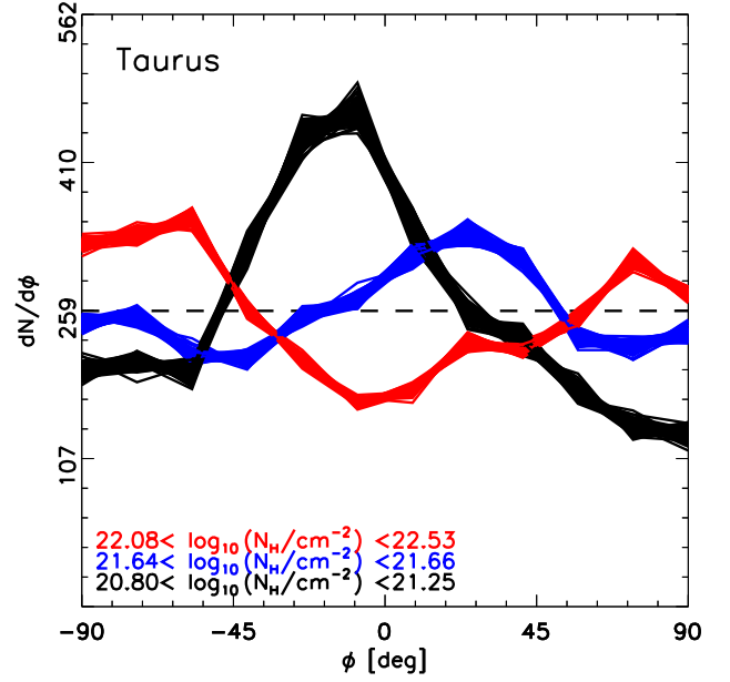
Fig. B.1. HROs in the Taurus region that correspond to the indicated N_H bins. The plotted values are obtained using the original \tau_{353} map at 10' resolution and maps of the Stokes parameters Q_r and U_r , which correspond to 1000 random noise realizations. Each realization is generated using a Gaussian probability density function centred on the measured values Q and U with variances \sigma_Q^2 and \sigma_U^2 .
