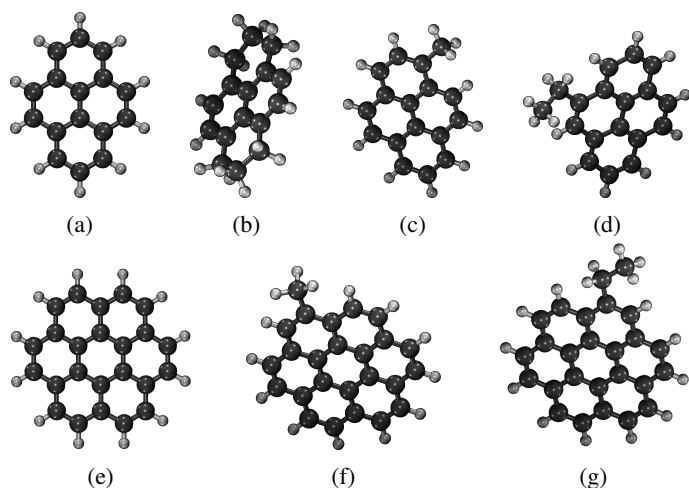
Fig. 1. Molecular structures, optimized with the GAUSSIAN16 package at the B3LYP/6-31g(d,p) level of theory, of cations of (a) pyrene ( C_{16}H_{10}^+ , Pyr^+ ), (b) 1,2,3,6,7,8-hexahydro-pyrene ( C_{16}H_{16}^+ , H_6-Pyr^+ ), (c) 1-methyl-pyrene ( C_{17}H_{12}^+ , MePyr^+ ), (d) 4-ethyl-pyrene ( C_{18}H_{14}^+ , EtPyr^+ ), (e) coronene ( C_{24}H_{12}^+ , Cor^+ ), (f) methyl-coronene ( C_{25}H_{14}^+ , MeCor^+ ), and (g) ethyl-coronene ( C_{26}H_{16}^+ , EtCor^+ ).
