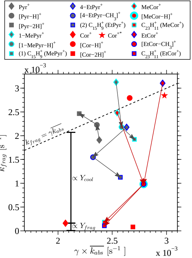
Fig. 10. Fragmentation rate of the studied species (apart H 6 -Pyr + ) as a function of the rescaled average absorption rate (by the \gamma factor, see text for details). The pyrene-based (resp. coronene-based) species are in gray (resp. red). The cyan (resp. blue) edge indicates the methylated (resp. ethylated) species. The dashed line corresponds to k_{\text{frag}} = \gamma k_{\text{abs}} . The fragmentation fraction ( Y_{\text{frag}} ) and the cooling fraction ( Y_{\text{cool}} ) are displayed for Cor + as an example. For MeCor + and EtCor + , the arrows point to the increased stability in the fragments formed by VUV processing. All the Y_{\text{cool}} values are given in Table 1.
