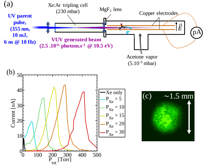
Fig. A.1. Characterization of the VUV source. (a) Setup to record the number of VUV photons generated per second. (b) Calibration for 10 mJ UV pulses. (c) Image of the VUV beam profile.
