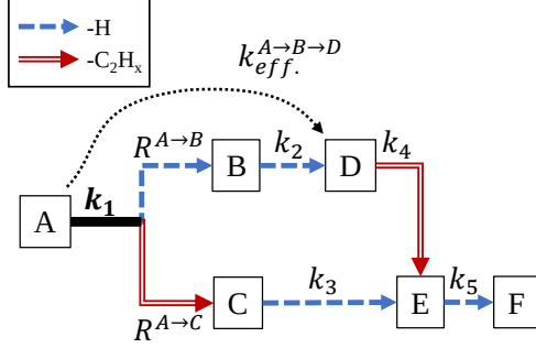
Fig. C.1. Example of a fragmentation map for an initial species ( A ) that dissociates into several fragments B , C , etc. The fragmentation rates ( k_i ) and the branching ratios ( R^{X→Y} ) permit us to compute the effective fragmentation rates ( k_{\text{eff}}^{A→M} ) and the total loss rates ( K_{\text{tot}}^{X-\text{loss}} ) corresponding to the loss of a given X neutral fragment (atom or molecular group).
