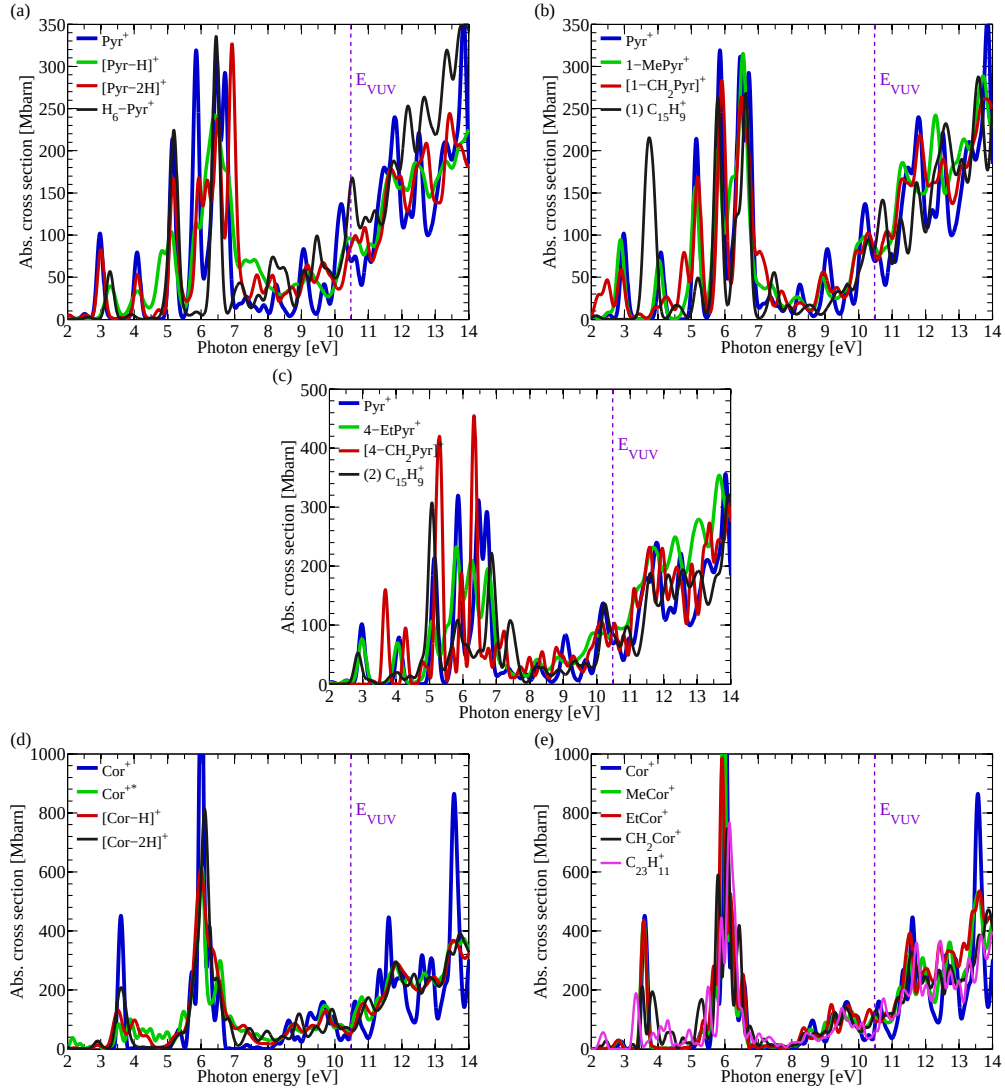
Fig. D.1. Photoabsorption cross sections calculated using TD-DFT for the studied parent cations and some of their relevant fragments: (a) \text{Pyr}^+ ( \text{H}_6\text{-Pyr}^+ also included), (b) 1\text{-MePyr}^+ , (c) 4\text{-EtPyr}^+ , (d) \text{Cor}^+ , and, (e) \text{MeCor}^+ and \text{EtCor}^+ .
