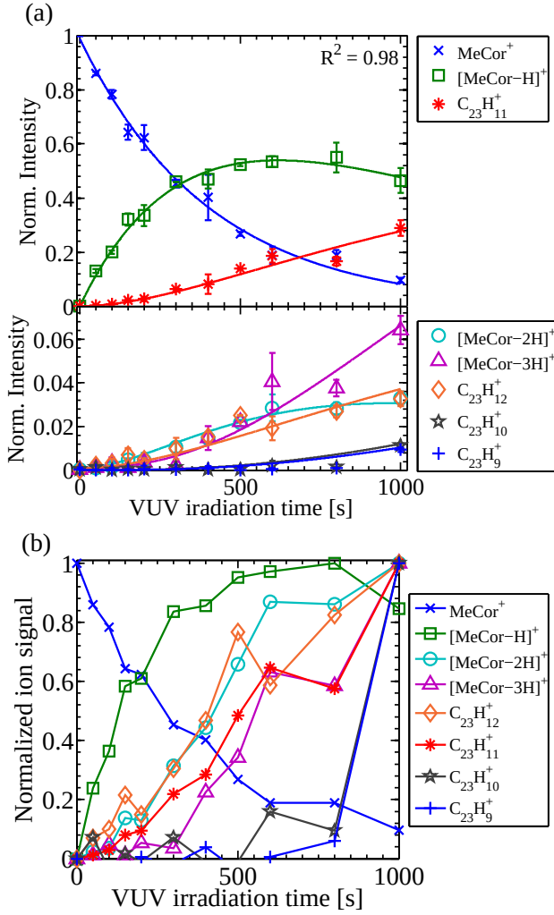
Fig. 4. VUV photoprocessing kinetic curves of MeCor + and its fragments. (a) Normalized intensity of each channel (defined by Eq. (1)) for VUV irradiation times up to 1000 s. Top panel: main channels Bottom panel: zoom on the minor channels. The solid curves correspond to the fitting functions that were derived with the procedure described in Sect. 2.4. (b) Normalized-to-one kinetic signal of each ion channel.
