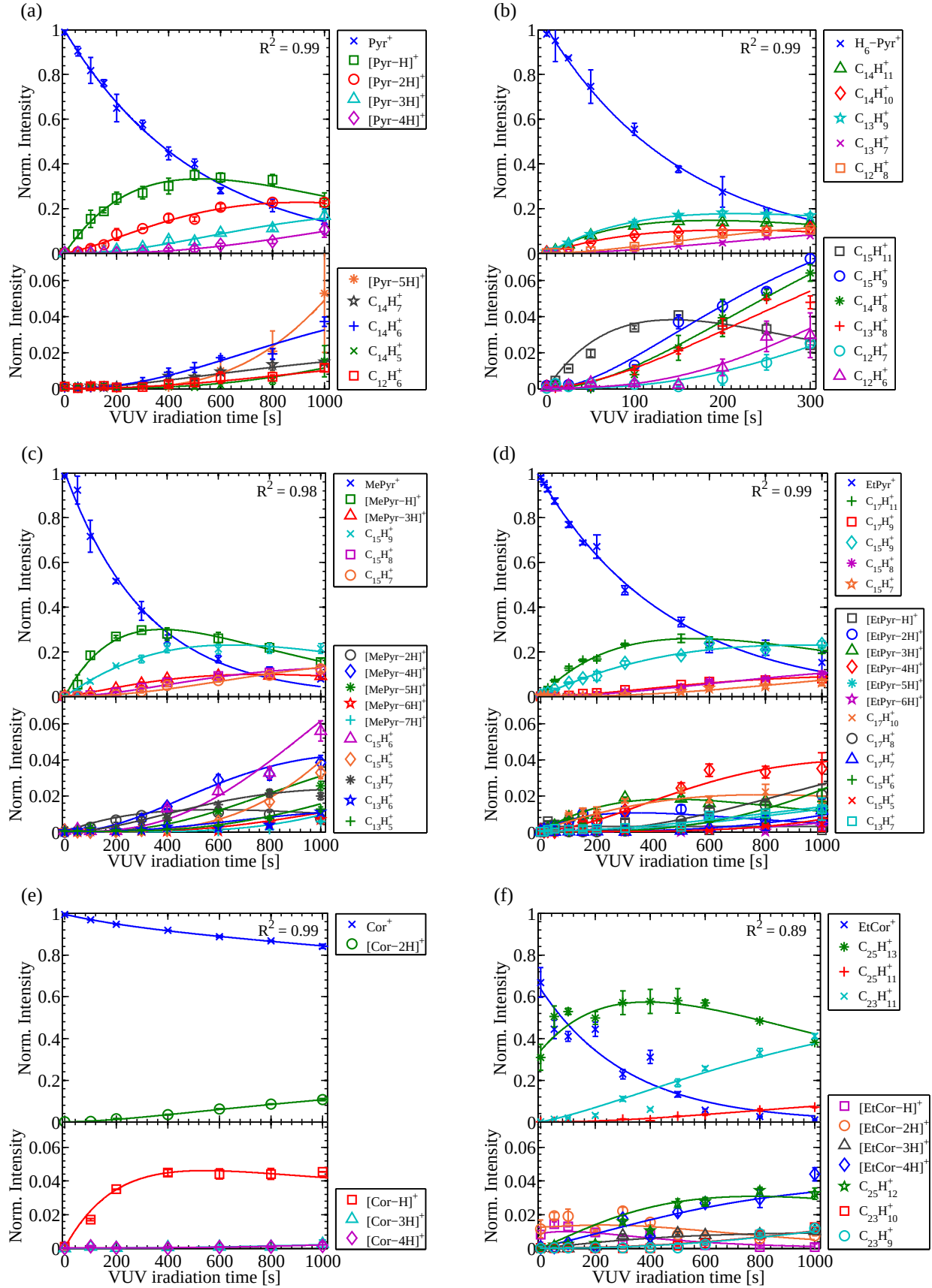
Fig. B.1. Kinetic curves of the studied PAH cations and their fragments: (a) Pyr + , (b) H 6 -Pyr + , (c) MePyr + , (d) EtPyr + , (e) Cor + , (f) EtCor + (MeCor + is shown in Fig. 4a). For each figure, the top panel shows the main channels while the bottom panel is a zoom on the minor channels. The solid curves correspond to the fitting functions that were derived with the procedure described in Sect. 2.4. The derived photofragmentation maps are shown in Figs. 6, 8, and 9.
