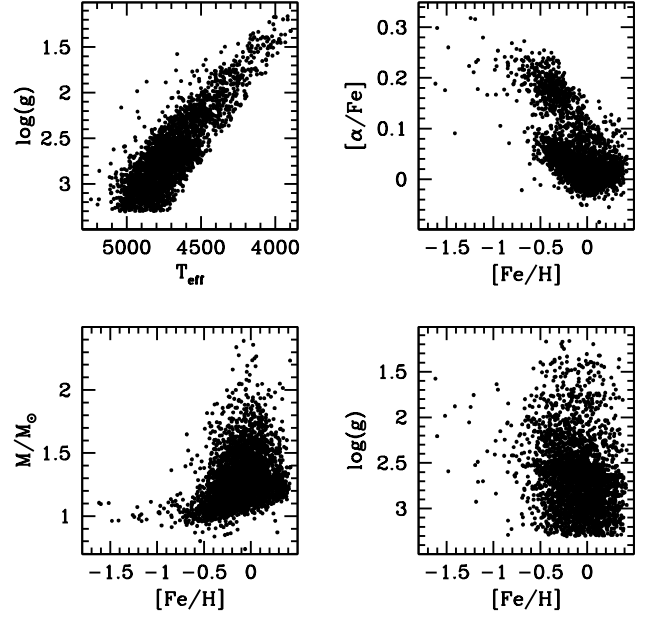
Fig. 1. The sample of RGB stars from the APOKASC dataset displayed in various diagrams: \log(g) - T_{eff} , [\alpha/Fe] - [Fe/H] , mass – [Fe/H] and \log(g) - [Fe/H] .
