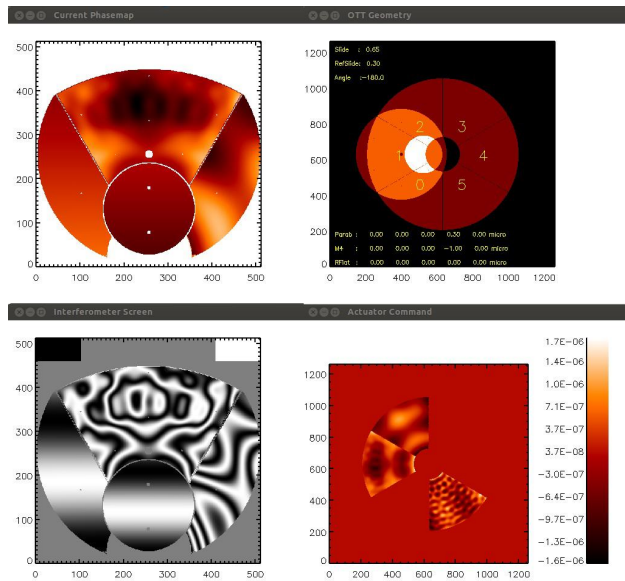
Figure 7. OTT phasemap with the parabola viewing at segment 1.
