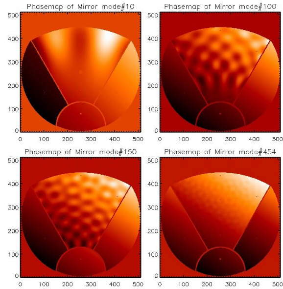
Figure 8. A sample of mirror modes measured on segment 1, including the differential piston from interferometer phase ambiguity.
