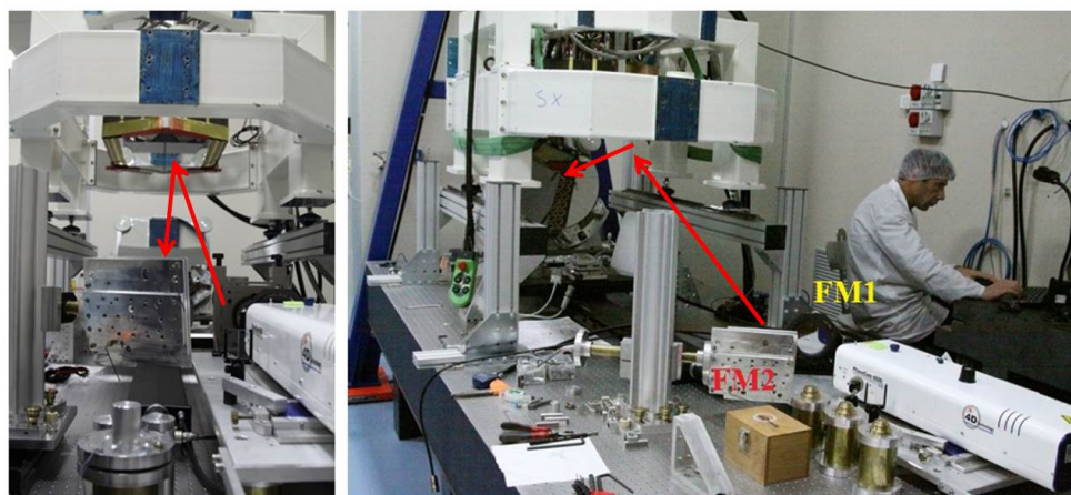
Figure 2. Optical bench for the measurement of the M4DP.
