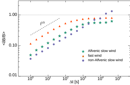
Fig. 6. Average value of \delta B/B from inertial to large scales, for fast (red triangles), Alfvénic slow (green stars), and non-Alfvénic slow (violet circles) winds.
