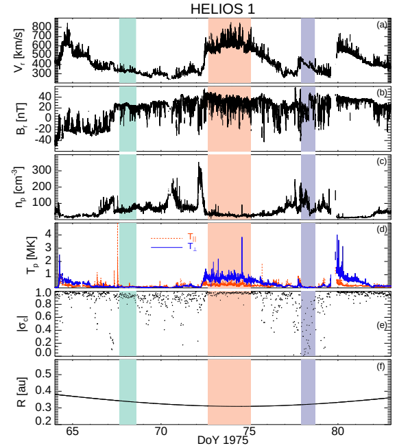
Fig. 1. Overview of solar wind data at the perihelion of Helios1 in 1975. (a) Radial component of the velocity; (b) radial component of the magnetic field; (c) proton density; (d) proton temperature: T_{\parallel} (red dashed line) and T_{\perp} (blue solid line); (e) absolute value of the 30 min averaged cross-helicity; (f) radial distance. The coloured bands denote the three different regimes of solar wind, namely Alfvénic slow (green), fast (orange), and non-Alfvénic slow (violet) winds.
