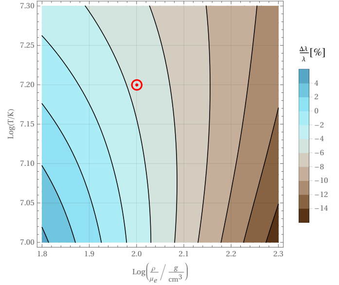
Fig. 1. Fractional variation of the {}^7\text{Be} electron-capture rate, \Delta\lambda/\lambda [\%] = 100 \cdot (R_{\text{STPB13}} - R_{\text{ADE11}})/R_{\text{ADE11}} , as a function of \rho/\mu_e and T , adopting the Simonucci et al. (2013) rate, as compared to that of Adelberger et al. (2011) for the PLJ14 solar composition (see Sect. 2). The solar core conditions are highlighted with the common solar symbol.
