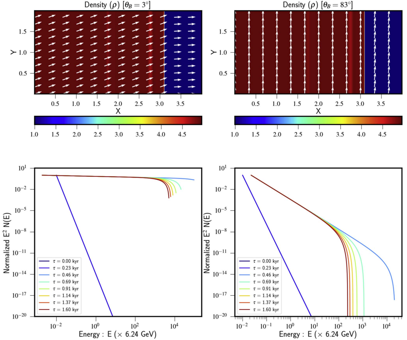
Figure 4. Top panels: density distribution in color at time t = 0.98 \text{ kyr} along with magnetic field vectors shown as white arrows for the quasi-parallel case \theta_B = 3^\circ (left) and quasi-perpendicular case \theta_B = 83^\circ (right) for the relativistic planar shock test. Bottom panels: the corresponding evolution of normalized spectral distribution of a representative macro-particle.
