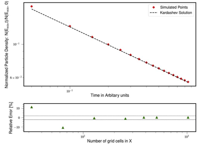
Figure 7. Top: comparison of the evolution with time (in arbitrary units) of a normalized spectral distribution, \mathcal{N}(E_{\min}, t) (red squares) with an analytical solution obtained from Equation (69) (black dashed line). Bottom: results from the convergence study with different resolution. The green triangles represent the relative errors (%) in estimating the analytical slope for the variation of \mathcal{N}(E_{\min}, t) with respect to time. The two black dashed lines mark the \pm 2\% error.
