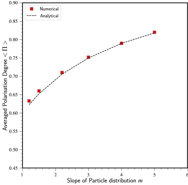
Figure 8. Comparison of the numerically estimated averaged ratio of J_{sy}(\nu) with J_{pol}(\nu) for \nu = 10^{10} GHz (red squares) with the theoretical values obtained from Equation (72) shown as the black dashed line.
